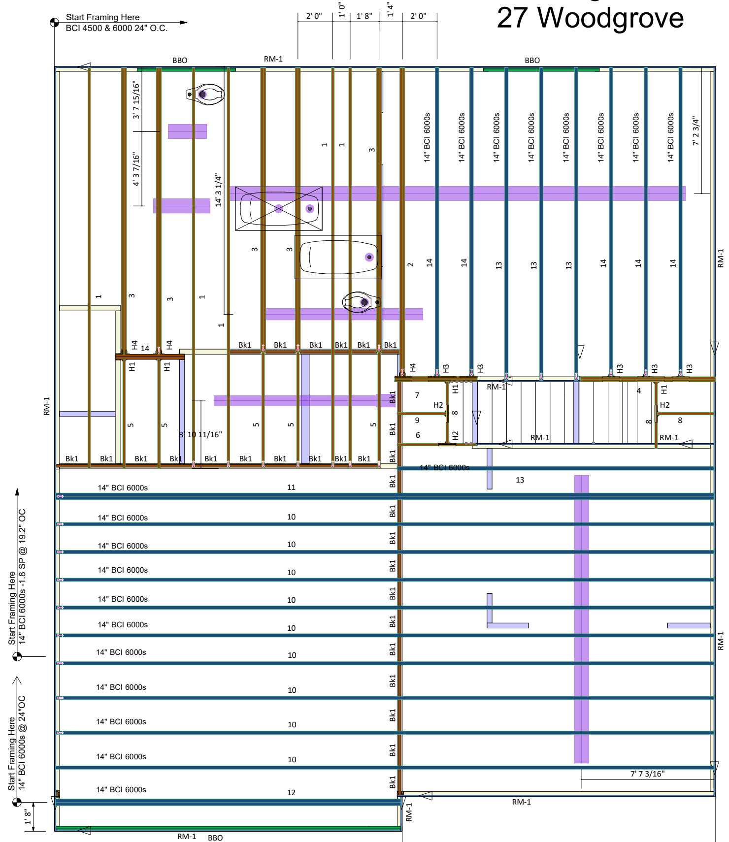
Second Floor Layout
