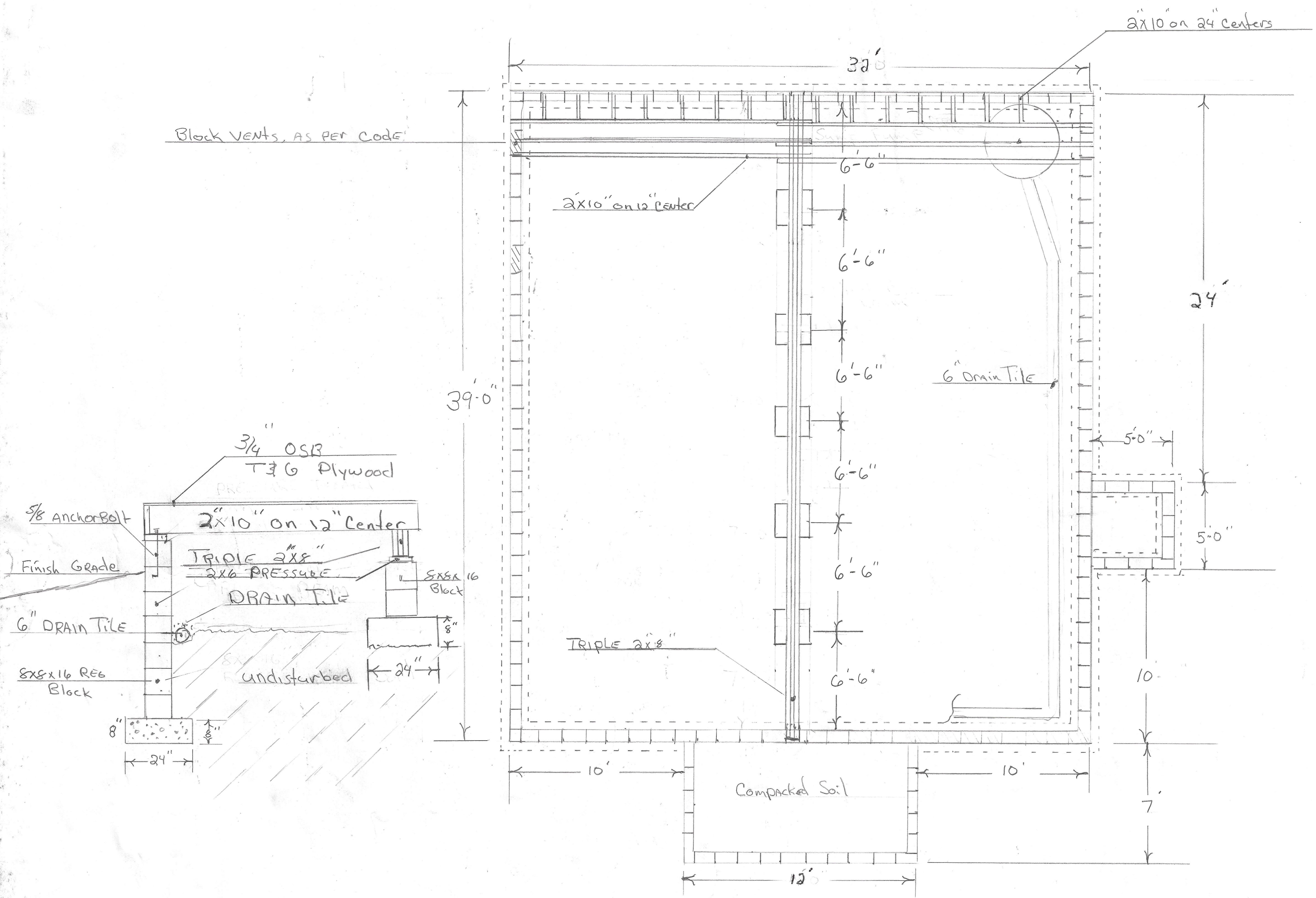
REVISED FOUNDATION DETAIL 291 PENDERGRAFT RD.
