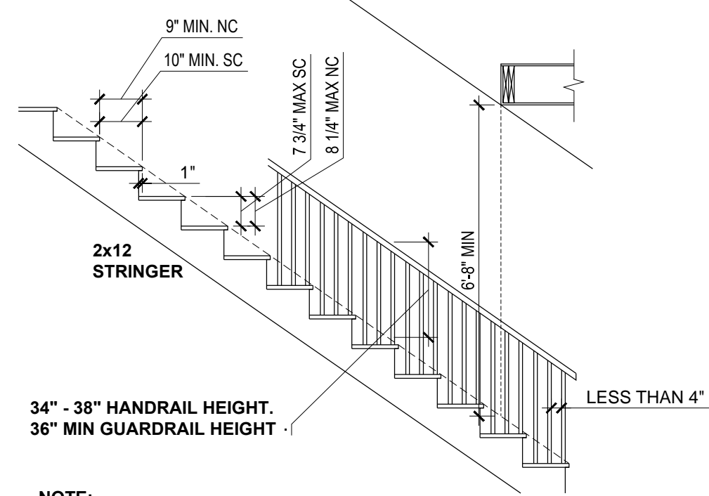
TYPICAL STAIR REQUIREMENTS 3/8" = 1'-0" 1
