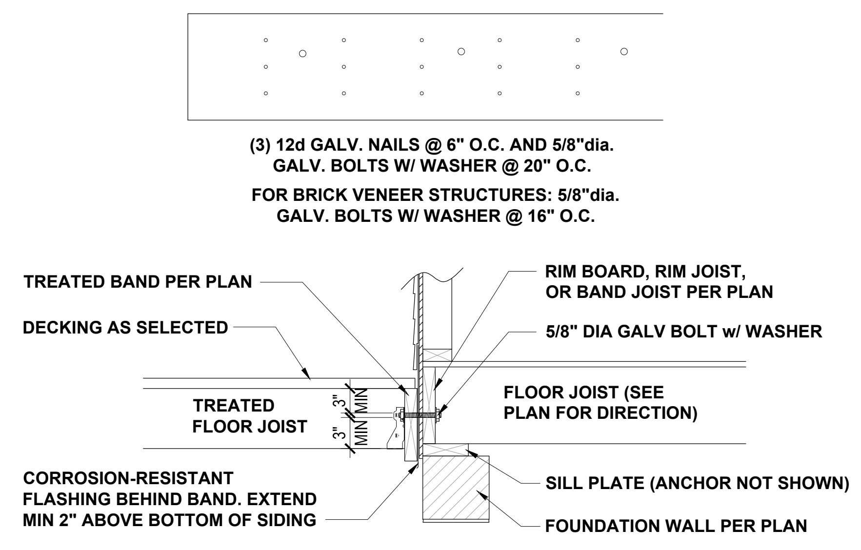
DECK ATTACHMENT 1/2" = 1'-0" 7
