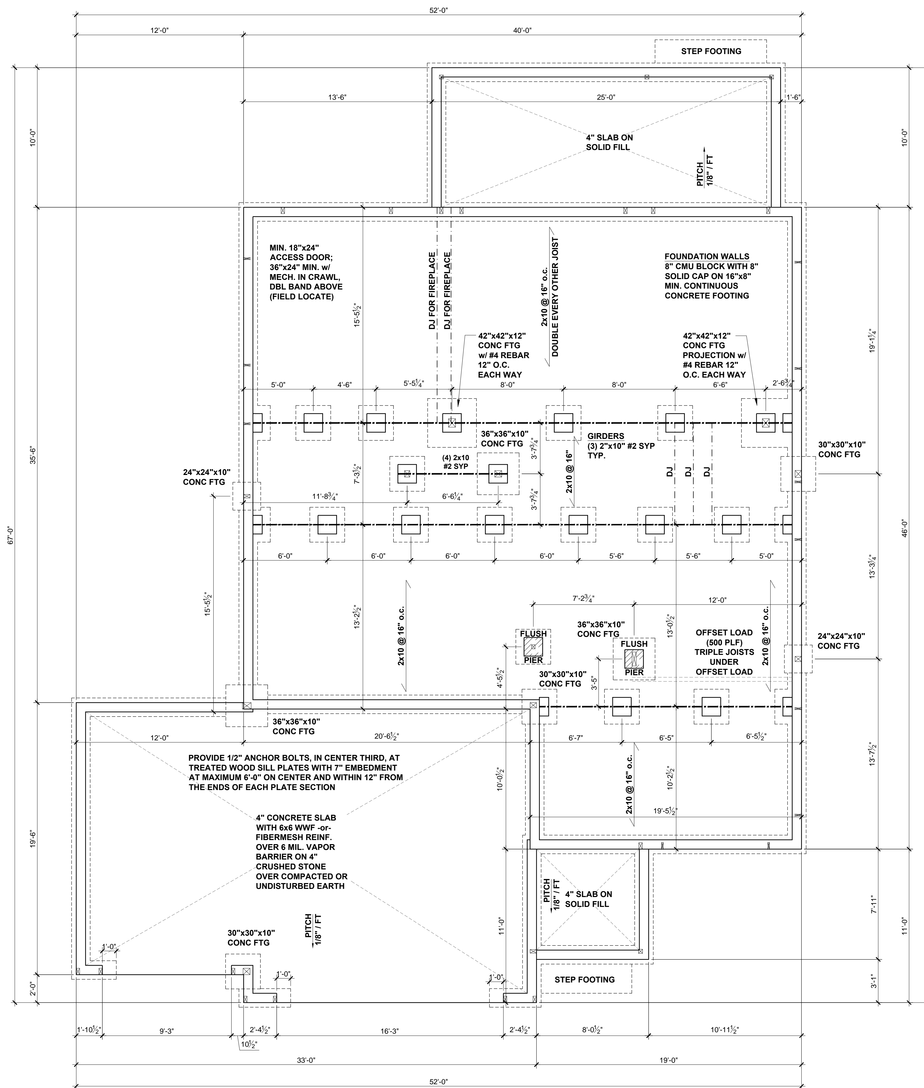
CRAWL SPACE FOUNDATION PLAN SCALE: 1/4"=1'-0"
