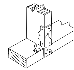
STANDARD INSTALLATION
