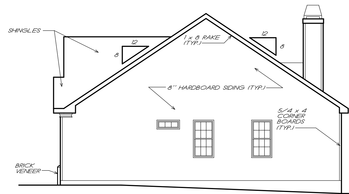
RIGHT ELEVATION 1/8" = 1'-0"
