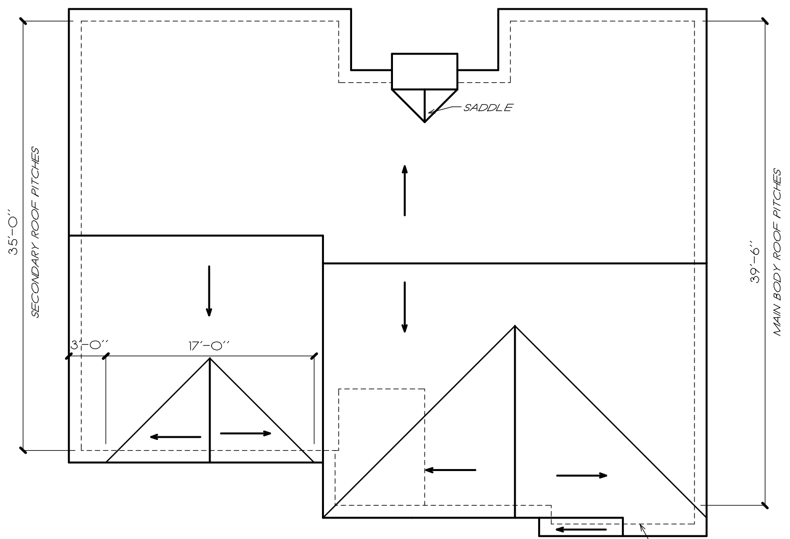
ROOF PLAN 1/8" = 1'-0"
