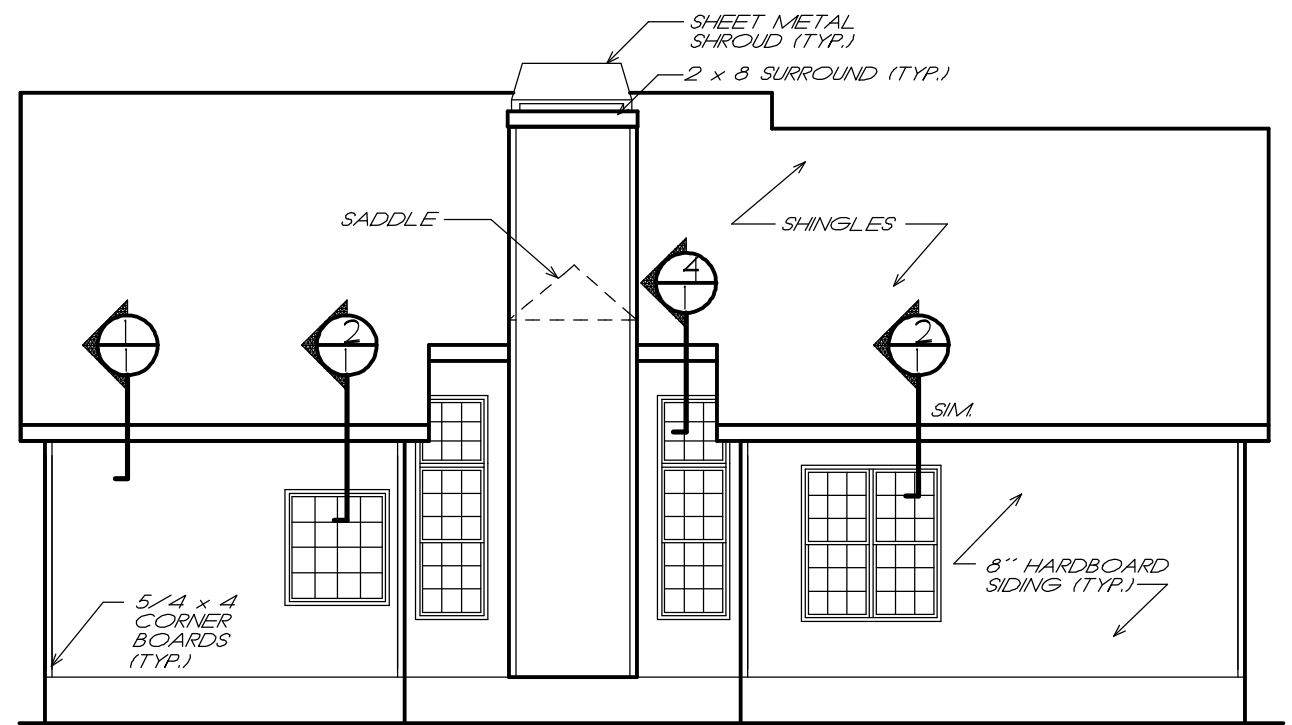
REAR ELEVATION 1/8" = 1'-0"
