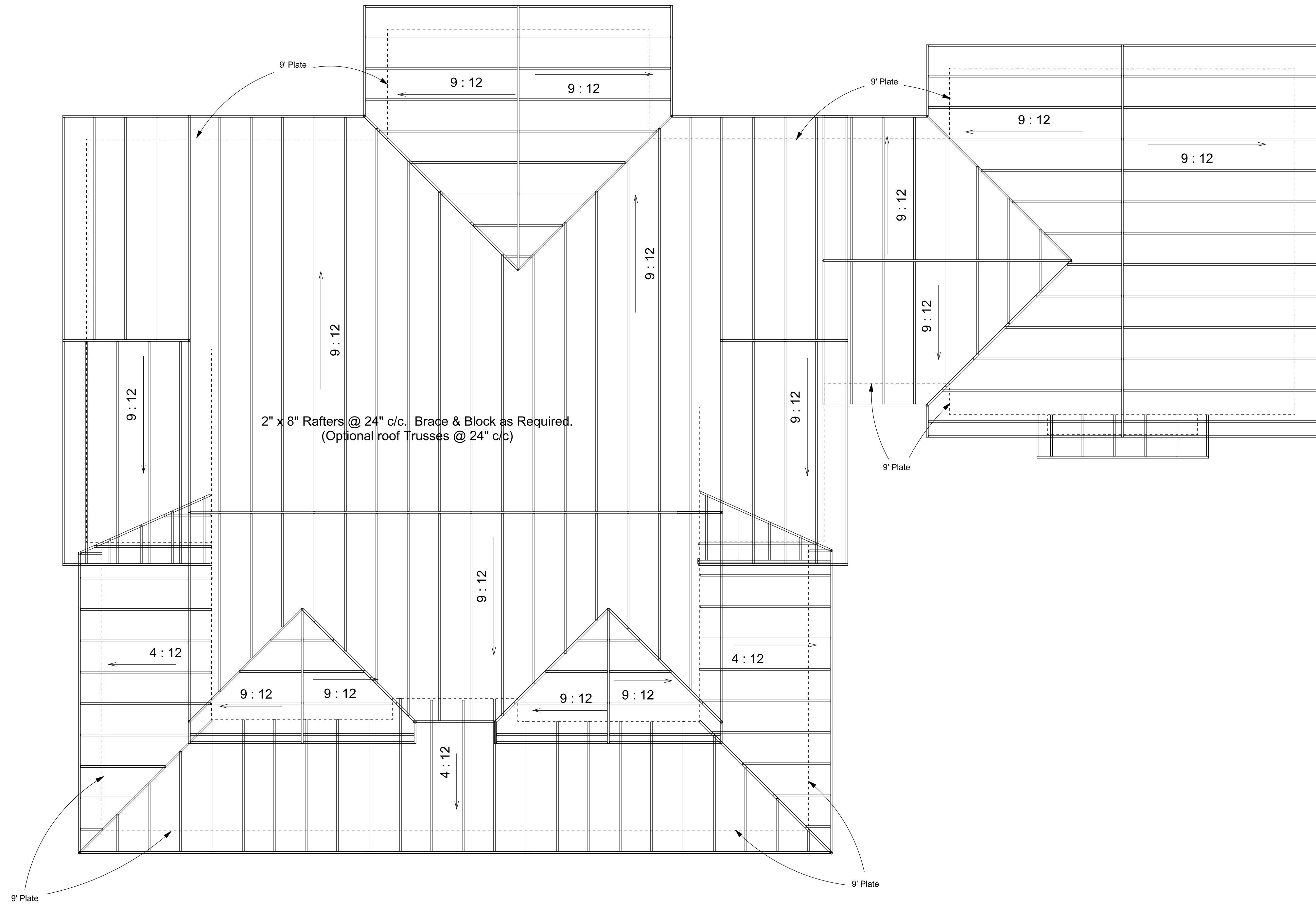
Roof Plan
