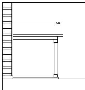
SCREENED PORCH PPO - RIGHT ELEVATION
