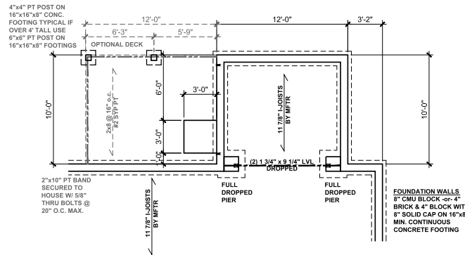
SUNROOM FOUNDATION
