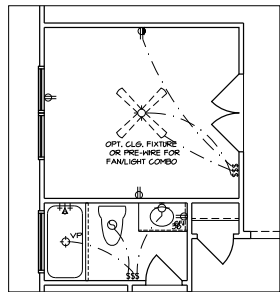
PPO - GROUND FLOOR ELECT. PLAN - CRAFTSMAN STUDY
