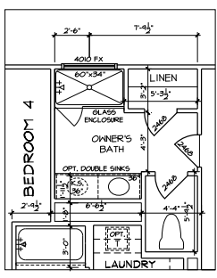
PPO - SECOND FLOOR PLAN STAND-IN SHOWER
