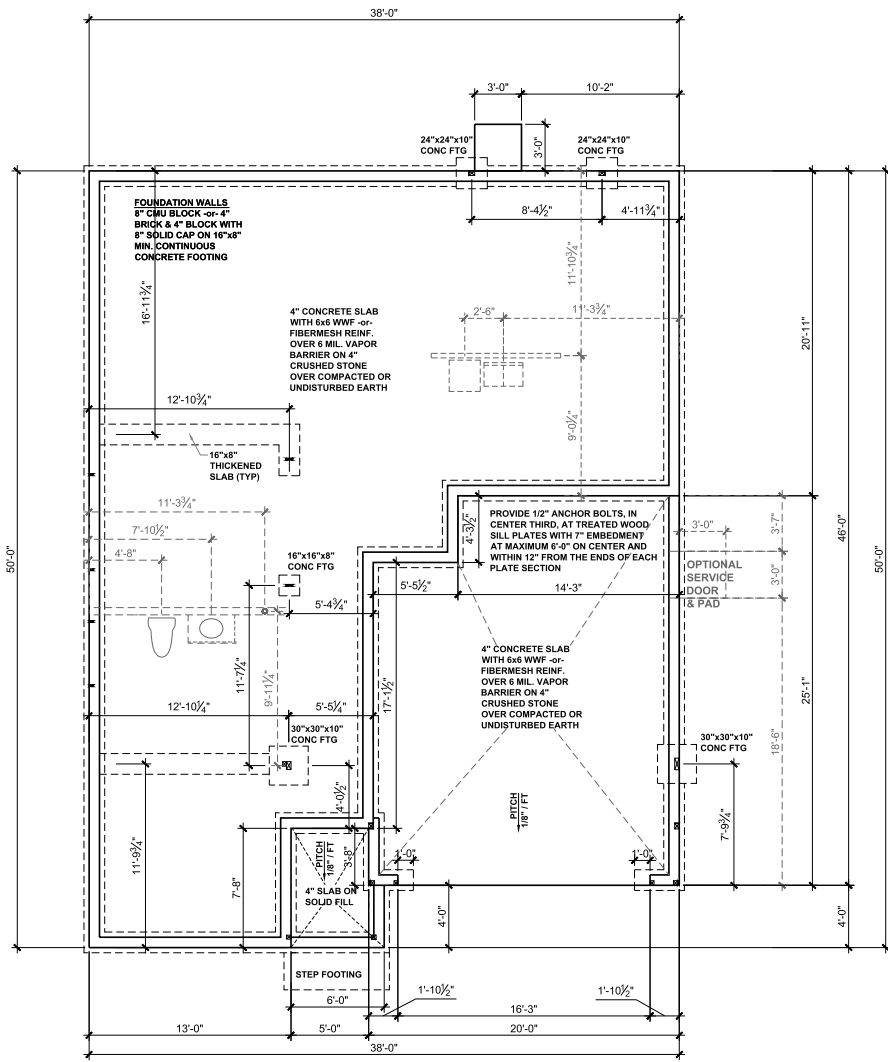
STEM WALL FOUNDATION PLAN - FARMHOUSE SCALE: 1/8" = 1'-0"
