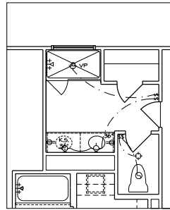
PPO - SECOND FLOOR ELECT. PLAN STAND-IN SHOWER
