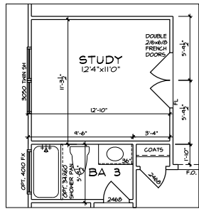
PPO - GROUND FLOOR PLAN - CRAFTSMAN STUDY
