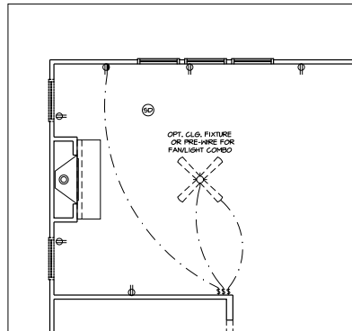
PPO - GROUND FLOOR ELECT. PLAN GAS FIREPLACE
