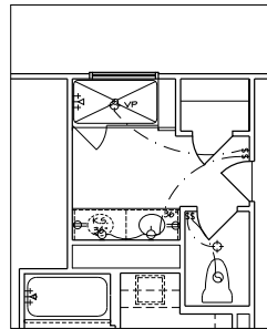
PPO - SECOND FLOOR ELECT. PLAN STAND-IN SHOWER w/ SEAT
