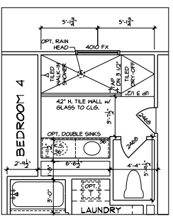
PPO - SECOND FLOOR PLAN BATH OASIS
