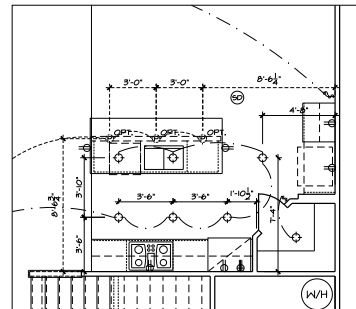
PPO - GROUND FLOOR ELECT. PLAN SIGNATURE KITCHEN
