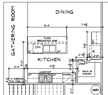
PPO - GROUND FLOOR PLAN SIGNATURE KITCHEN
