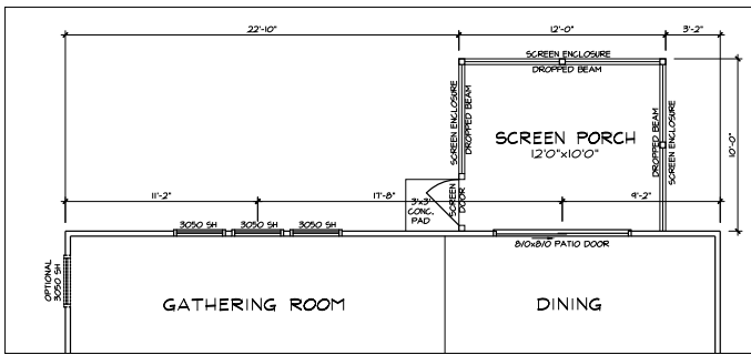
PPO - GROUND FLOOR PLAN SCREEN PORCH - RALEIGH
