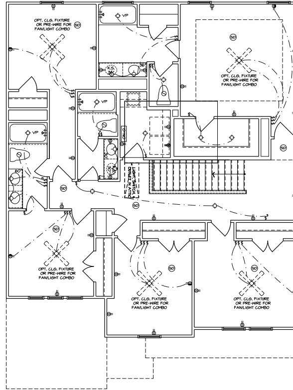
PPO - SECOND FLOOR ELECT. PLAN STAND-IN SHOWER
