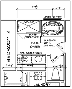
PPO - SECOND FLOOR PLAN BATH OASIS
