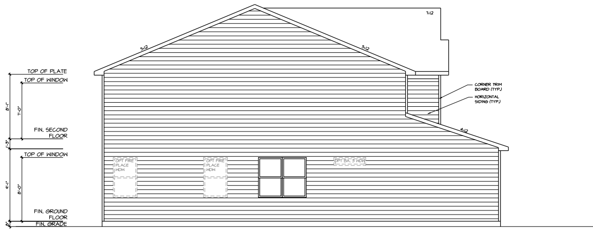
LEFT SIDE ELEVATION - FARMHOUSE
