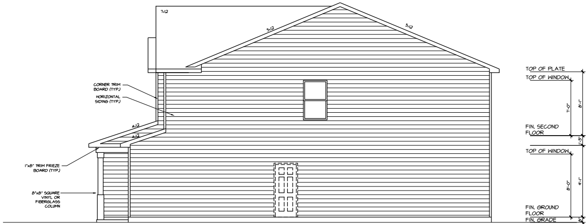
RIGHT ELEVATION - FARMHOUSE
