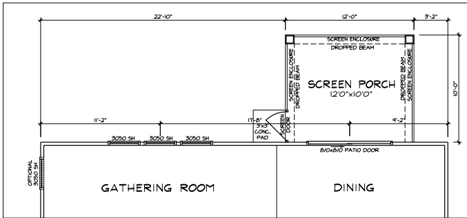
PPO - GROUND FLOOR PLAN SCREEN PORCH - CHARLOTTE
