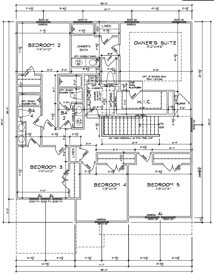
PPO - SECOND FLOOR PLAN STAND-IN SHOWER
