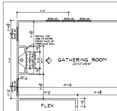
PPO - GROUND FLOOR PLAN GAS FIREPLACE
