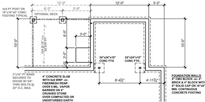
SUNROOM FOUNDATION
