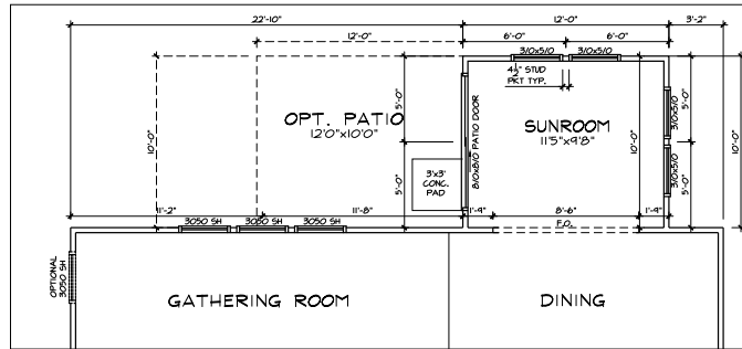
PPO - GROUND FLOOR PLAN SUNROOM
