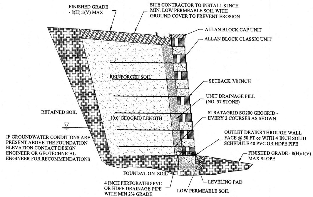
10.0 FEET MAXIMUM HEIGHT RETAINING WALL
