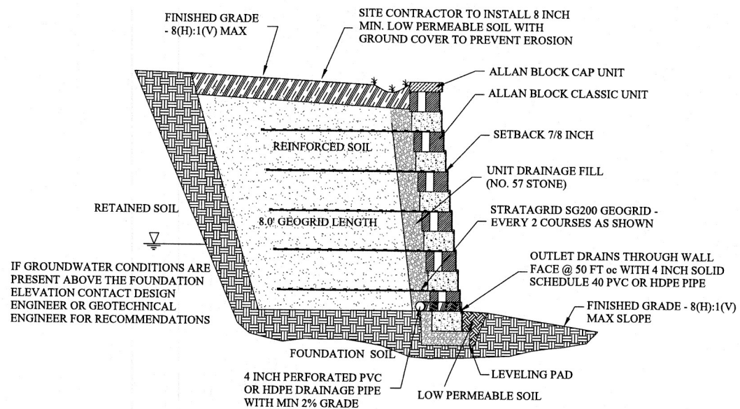
8.0 FEET MAXIMUM HEIGHT RETAINING WALL
