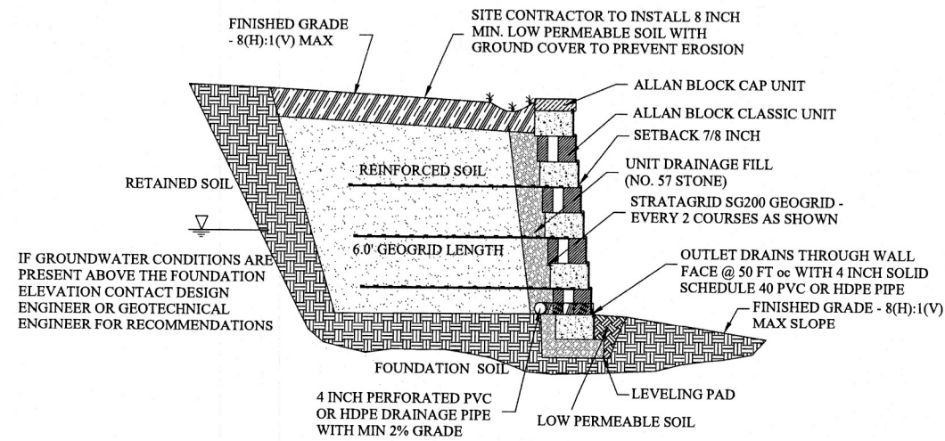
6.0 FEET MAXIMUM HEIGHT RETAINING WALL
