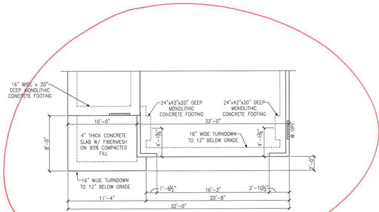
MONOLITHIC SLAB FOUNDATION PLAN ELEVATIONS 'B1' & 'B2'
