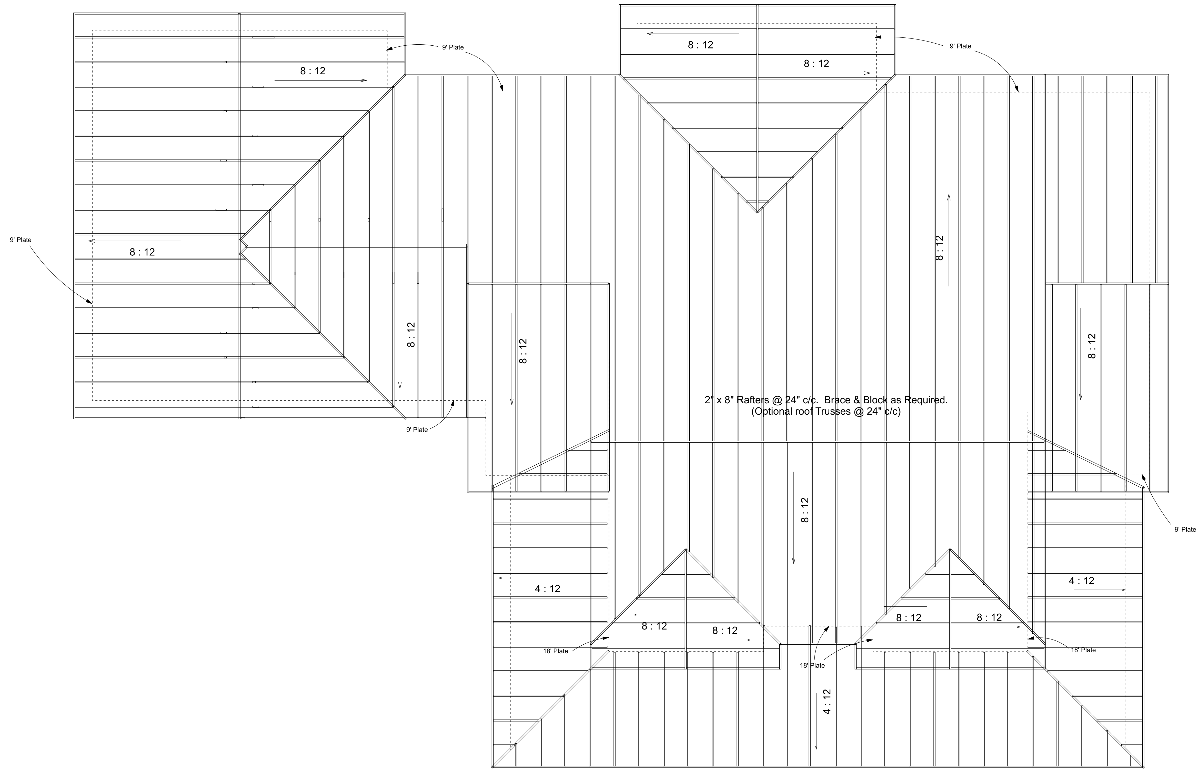
Roof Plan
