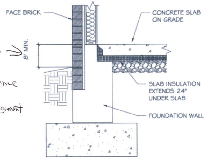
FIGURE O-5FRAME WALL
