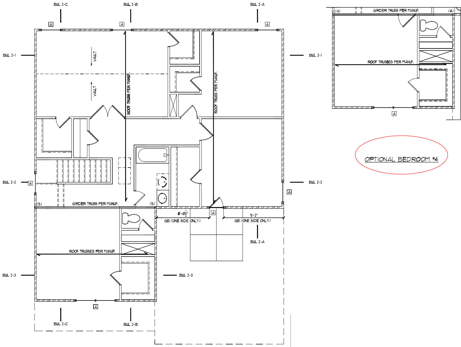
SECOND FLOOR FRAMING PLAN - ALL ELEVATIONS
