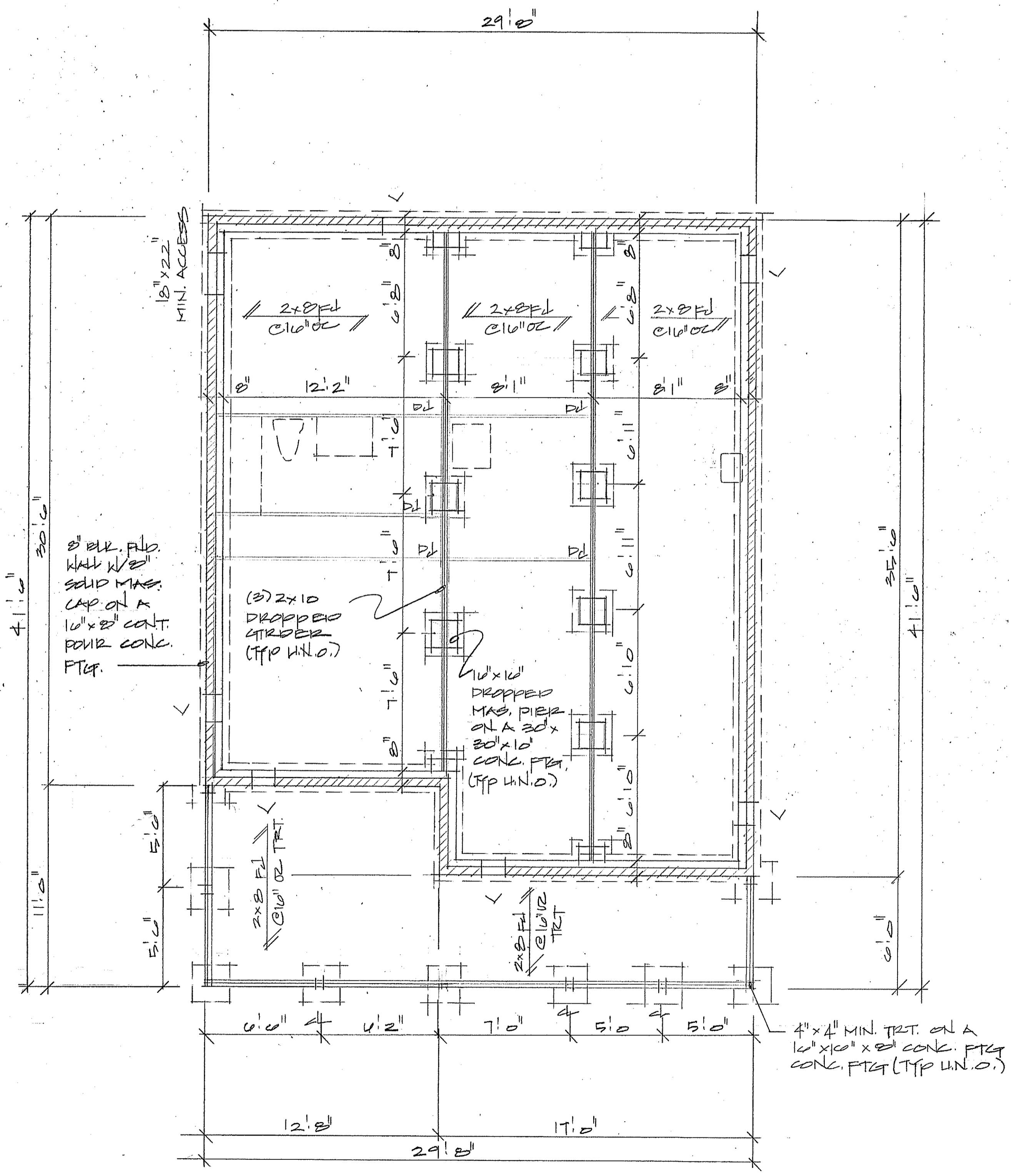
FOUNDATION PLAN @ 1/4" = 1'-0"
