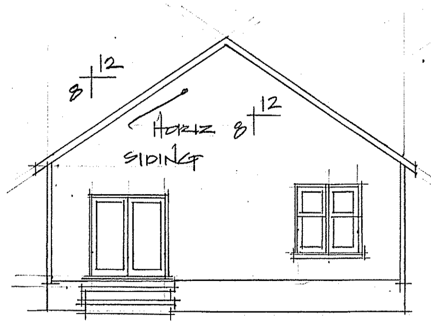
REAR ELEVATION @ 1/8" = 1'-0"
