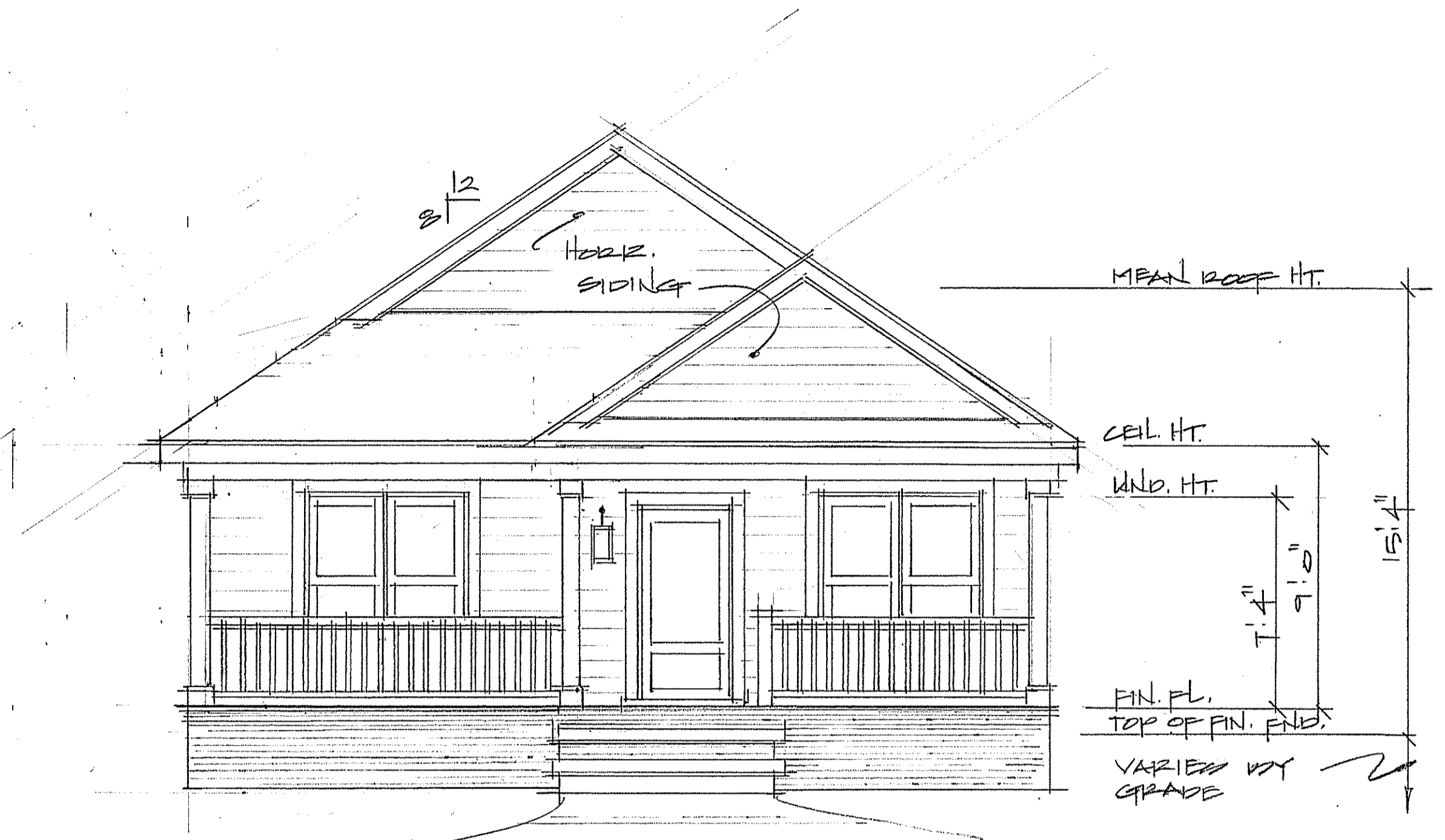
FRONT ELEVATION @ 1/4" = 1'-0"
