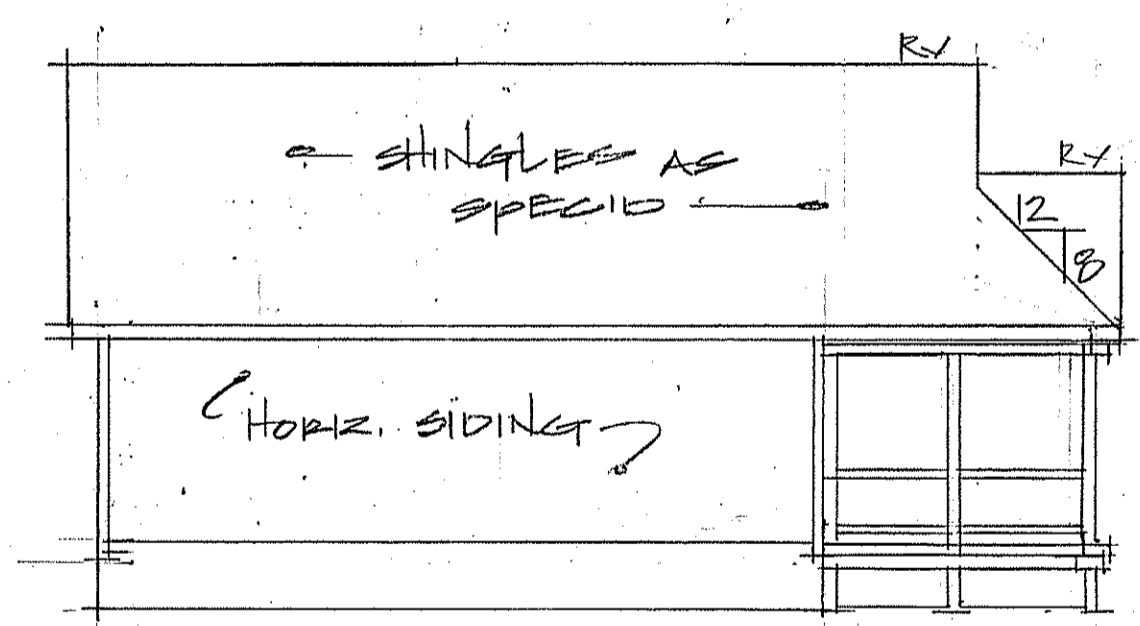
LEFT ELEVATION @ 1/8" = 1'-0"
