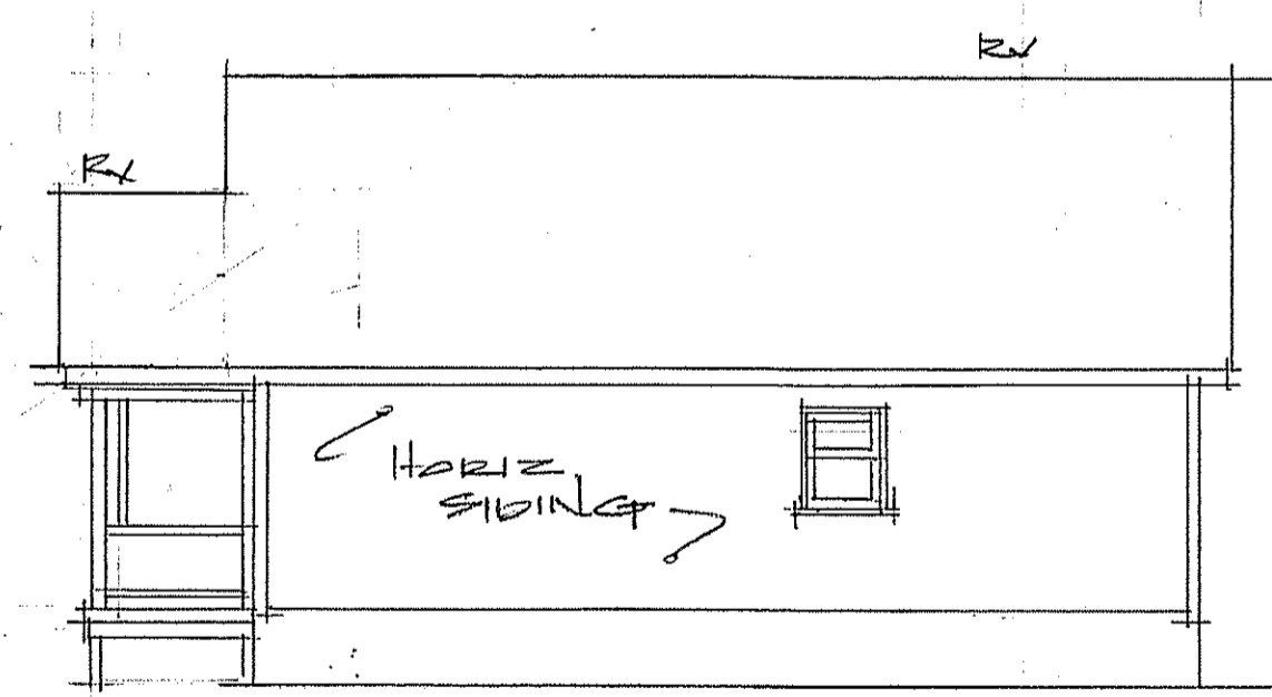
RIGHT ELEVATION @ 1/8" = 1'-0"
