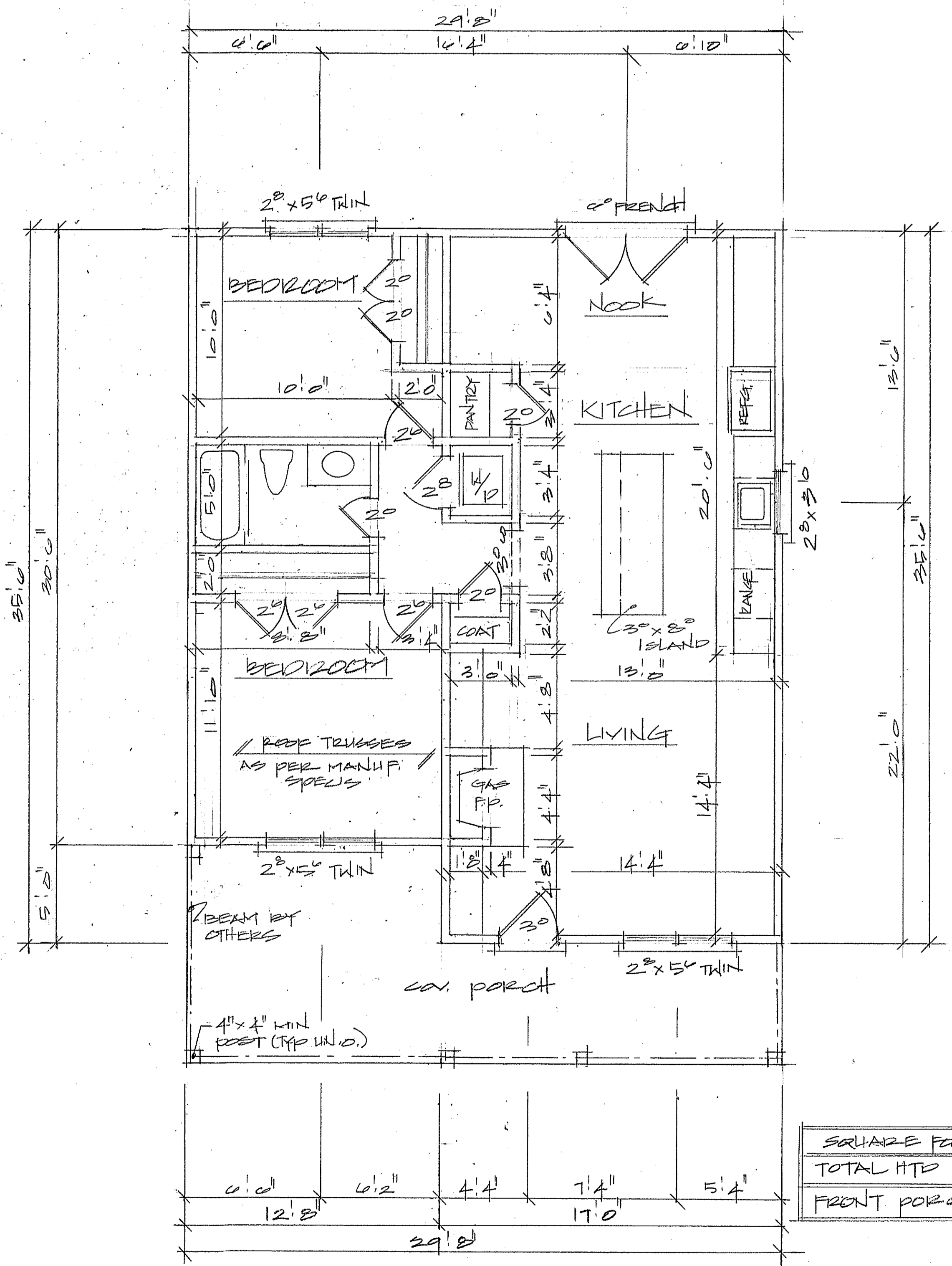
FLOOR PLAN @ 1/4" = 1'-0"
