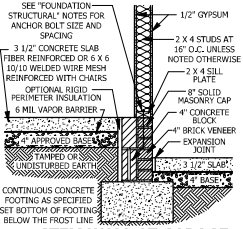
C STEM WALL AT GARAGE SCALE 1/2" = 1'-0"
