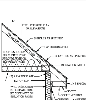
TYPICAL WALL DETAIL SCALE 3/4" = 1'-0"
