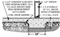
A STEM WALL SECTION SCALE 1/2" = 1'-0"
