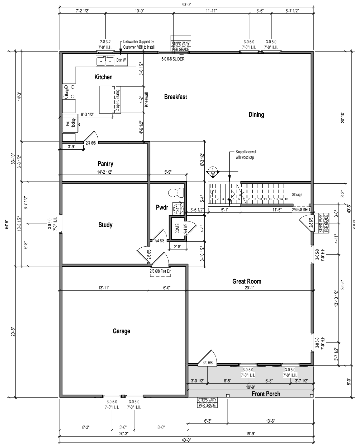
1 1st Floor Plan - Elev A 1/8" = 1'-0"
