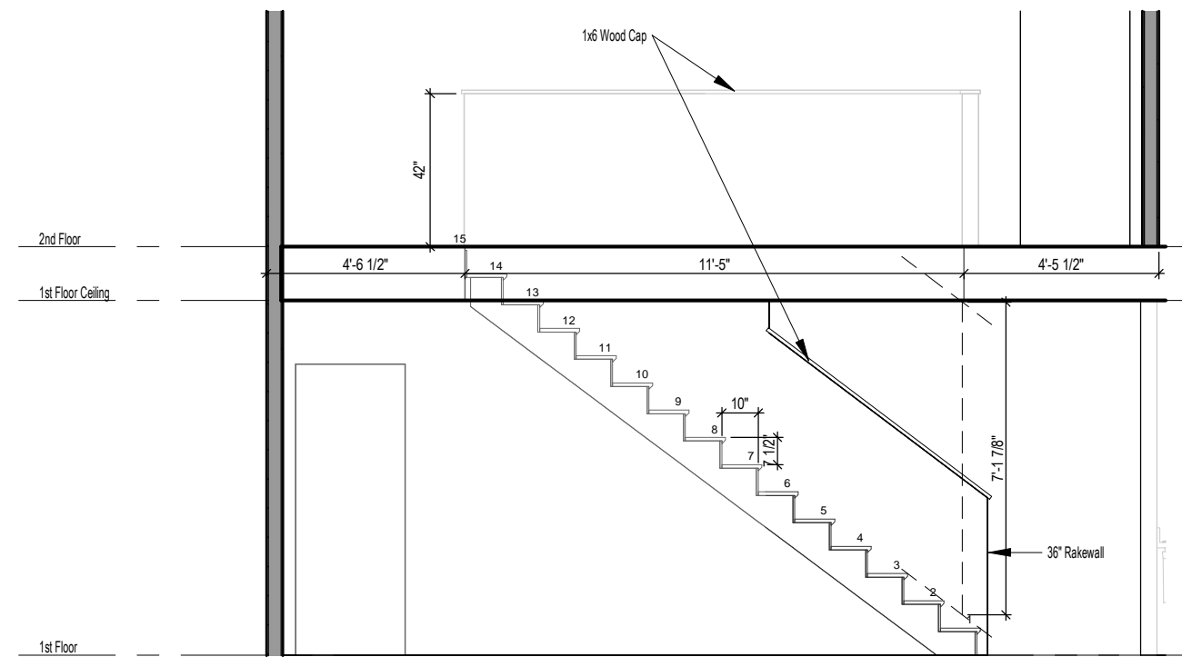
1 Stair Section 1/4" = 1'-0"
