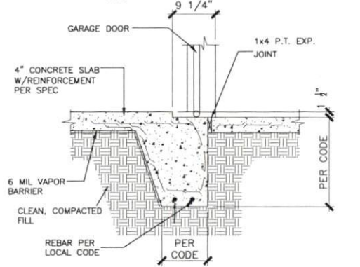
6 TYPICAL GARAGE DOOR DETAIL N.T.S.
