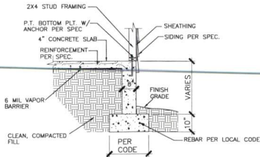
8 TYPICAL STEM WALL DETAIL N.T.S.
