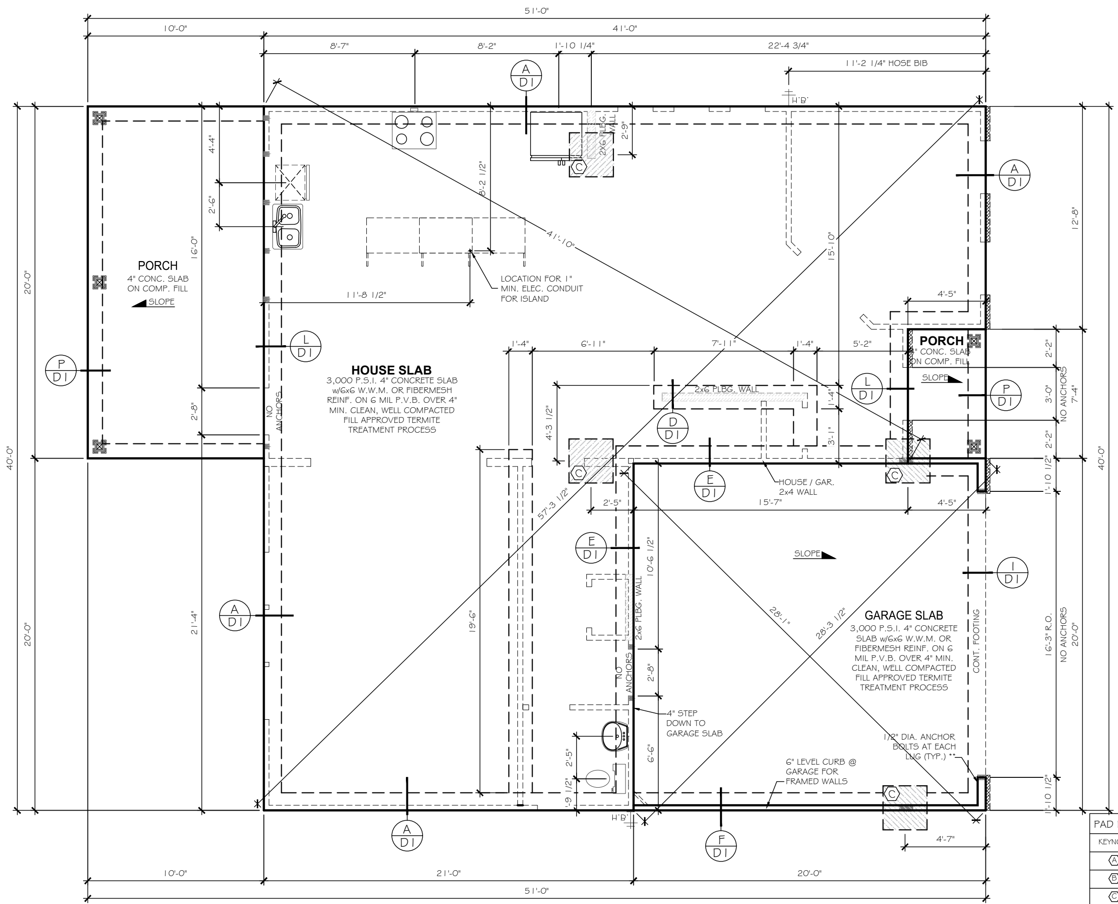
MONO SLAB FOUNDATION PLAN
