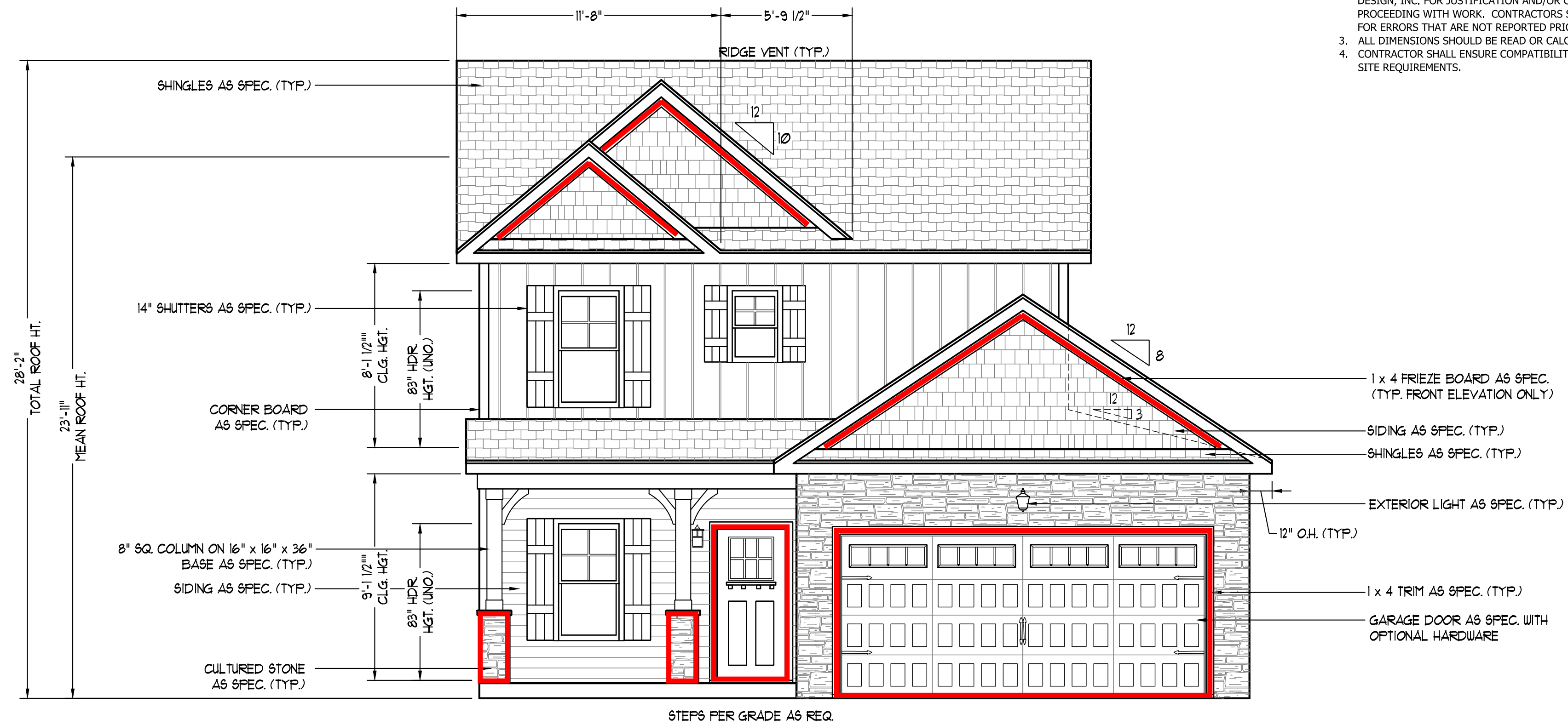
FRONT ELEVATION-C SCALE: 1/4" = 1'-0"
