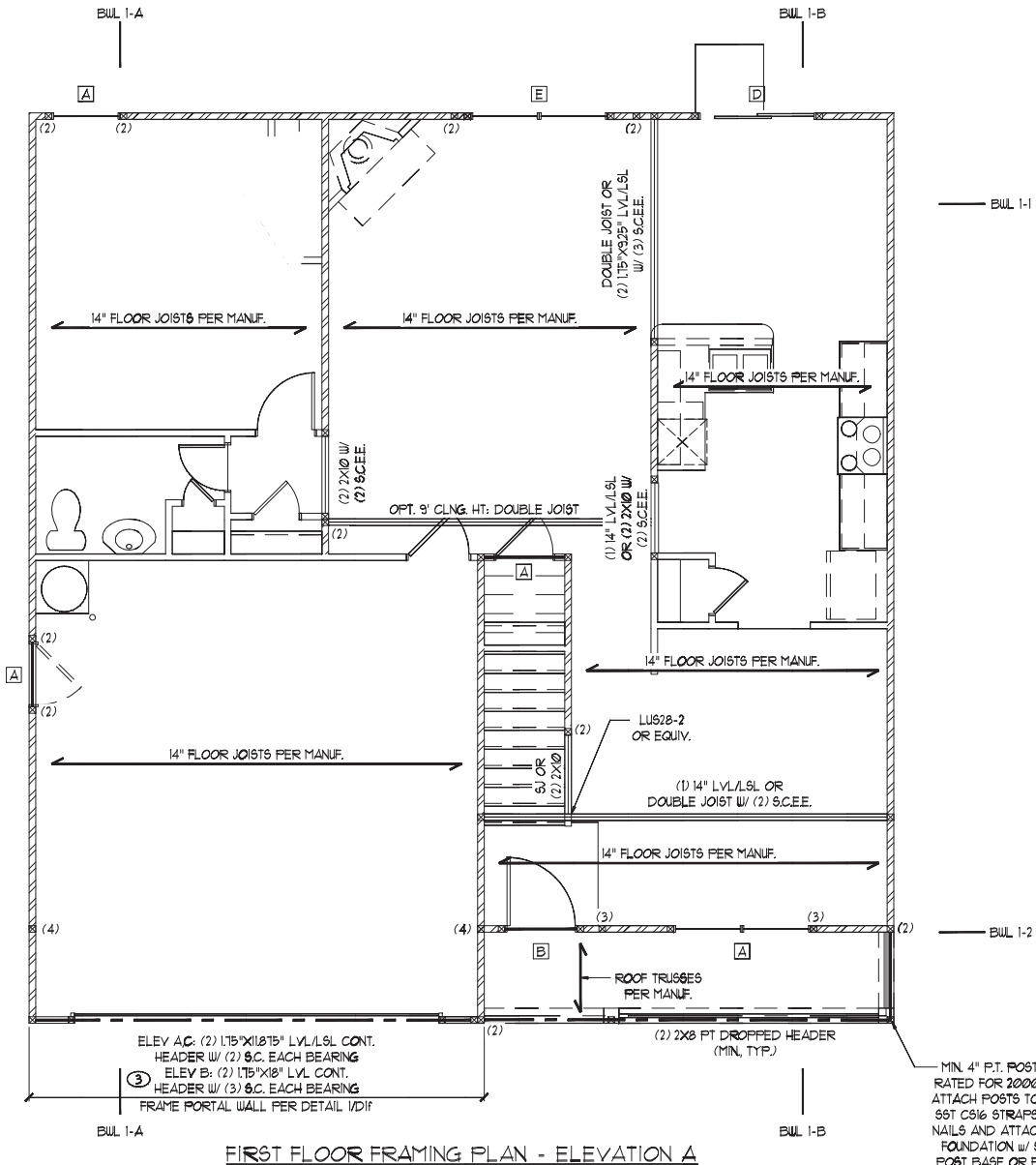
FIRST FLOOR FRAMING PLAN - ELEVATION A
