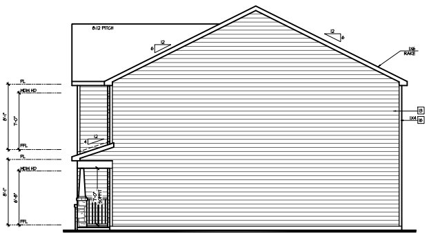
Right Elevation 'C' SCALE: 1/8"=1'-0" AT 22'X34' LAYOUT 1/8"=1'-0" AT 11'X11' LAYOUT
