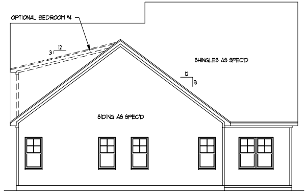
REAR ELEVATION SCALE: ----- 1/16" = 1'-0" WITH BEDROOM #4 OPTION
