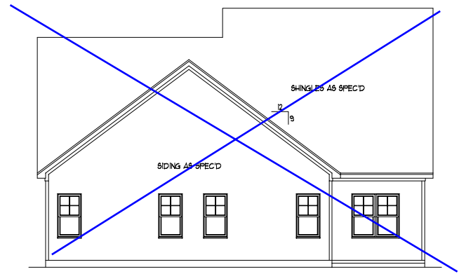
REAR ELEVATION SCALE: ----- 1/16" = 1'-0"
