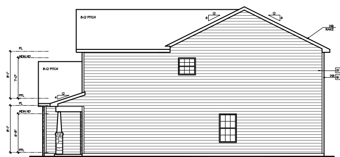
Right Elevation 'C' SCALE: 1/4"=1'-0" AT 22"x34" LAYOUT 1/8"=1'-0" AT 11"x17" LAYOUT
