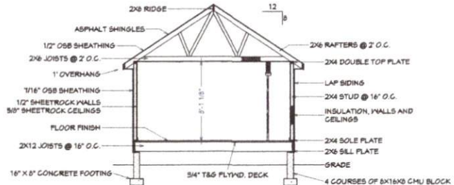
CROSS SECTION SCALE: 1/4" = 1'
