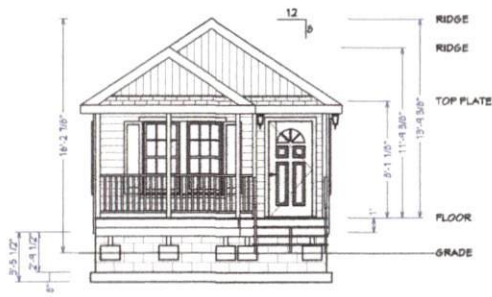
FRONT ELEVATION SCALE: 1/4" = 1'
