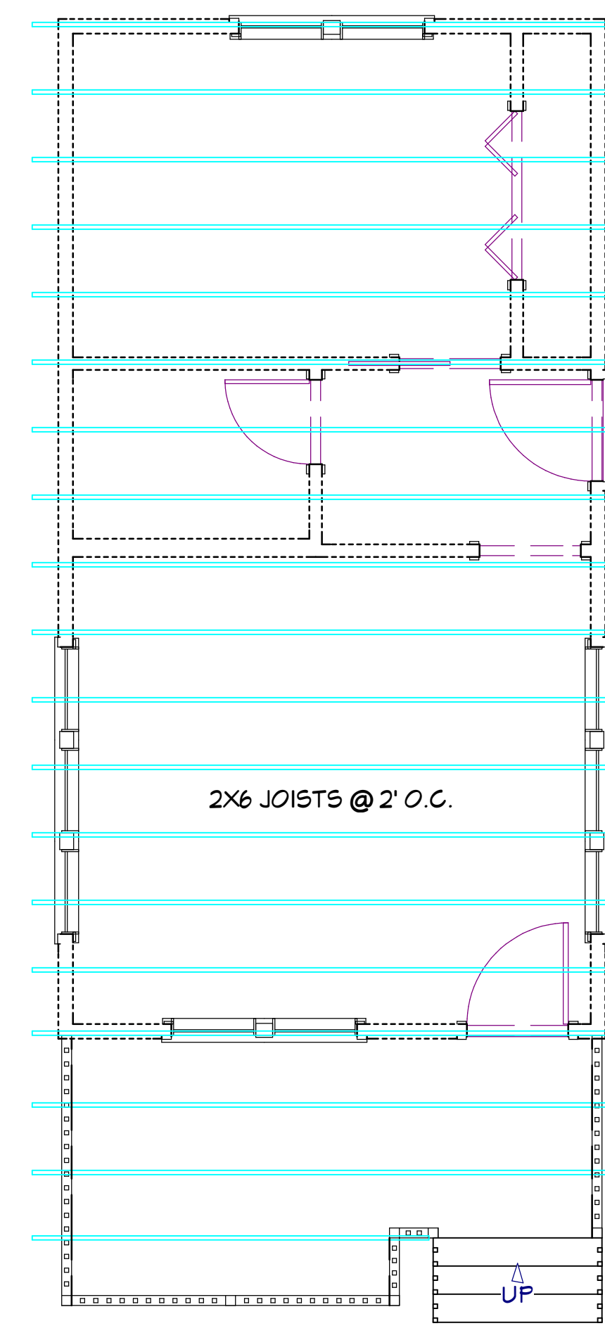
CEILING FRAMING PLAN SCALE: 1/4" = 1'
