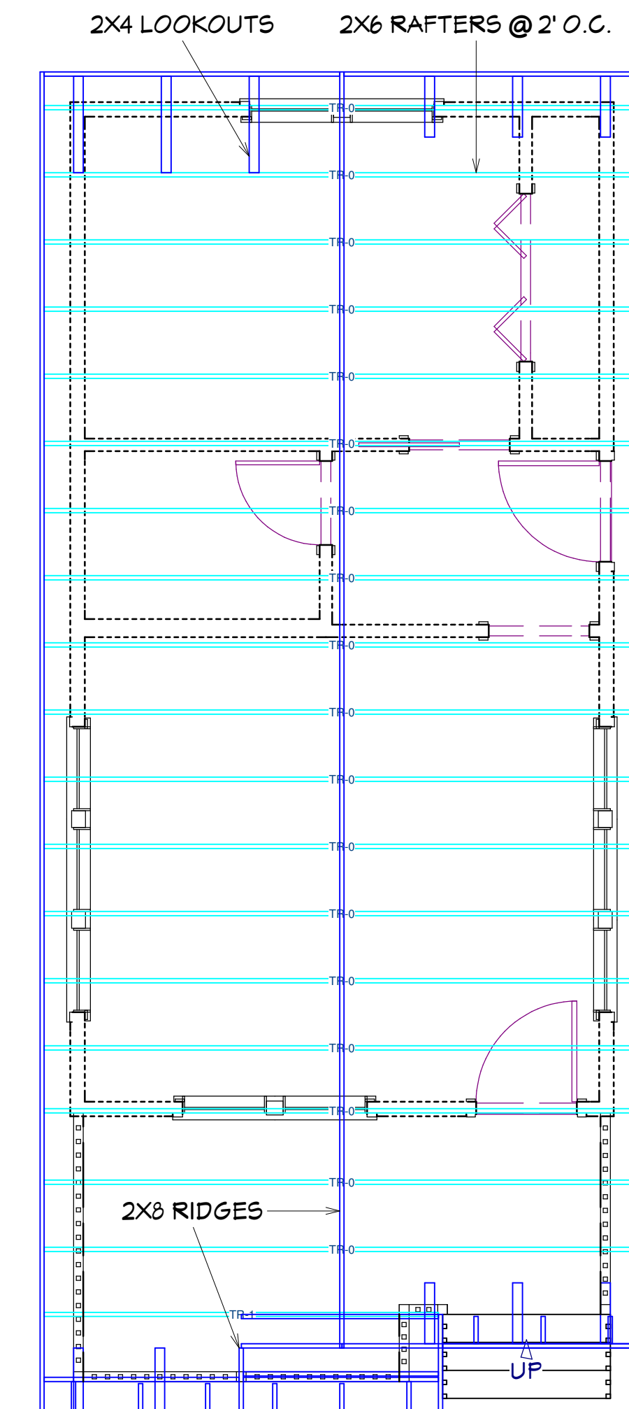
ROOF FRAMING PLAN SCALE: 1/4" = 1'
