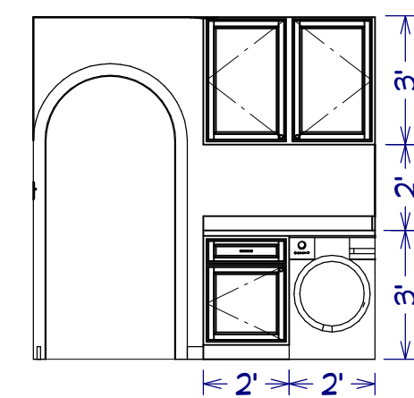
CABINET ELEVATION B SCALE: 1/4" = 1'
