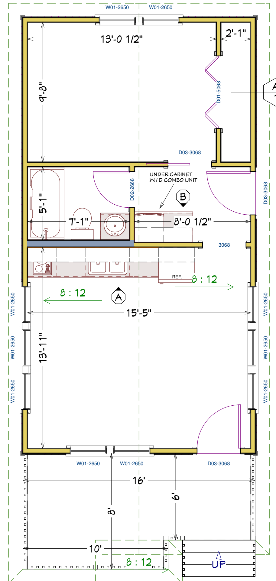
MAIN FLOOR PLAN SCALE: 1/4" = 1'
