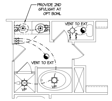
Opt Owner's Bath SCALE: 1/4"=1'-0" AT 22"X34" LAYOUT 1/8"=1'-0" AT 11"X11" LAYOUT
