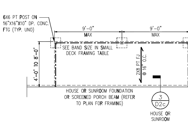
TYP. SMALL REAR DECK PLAN N.T.S.
