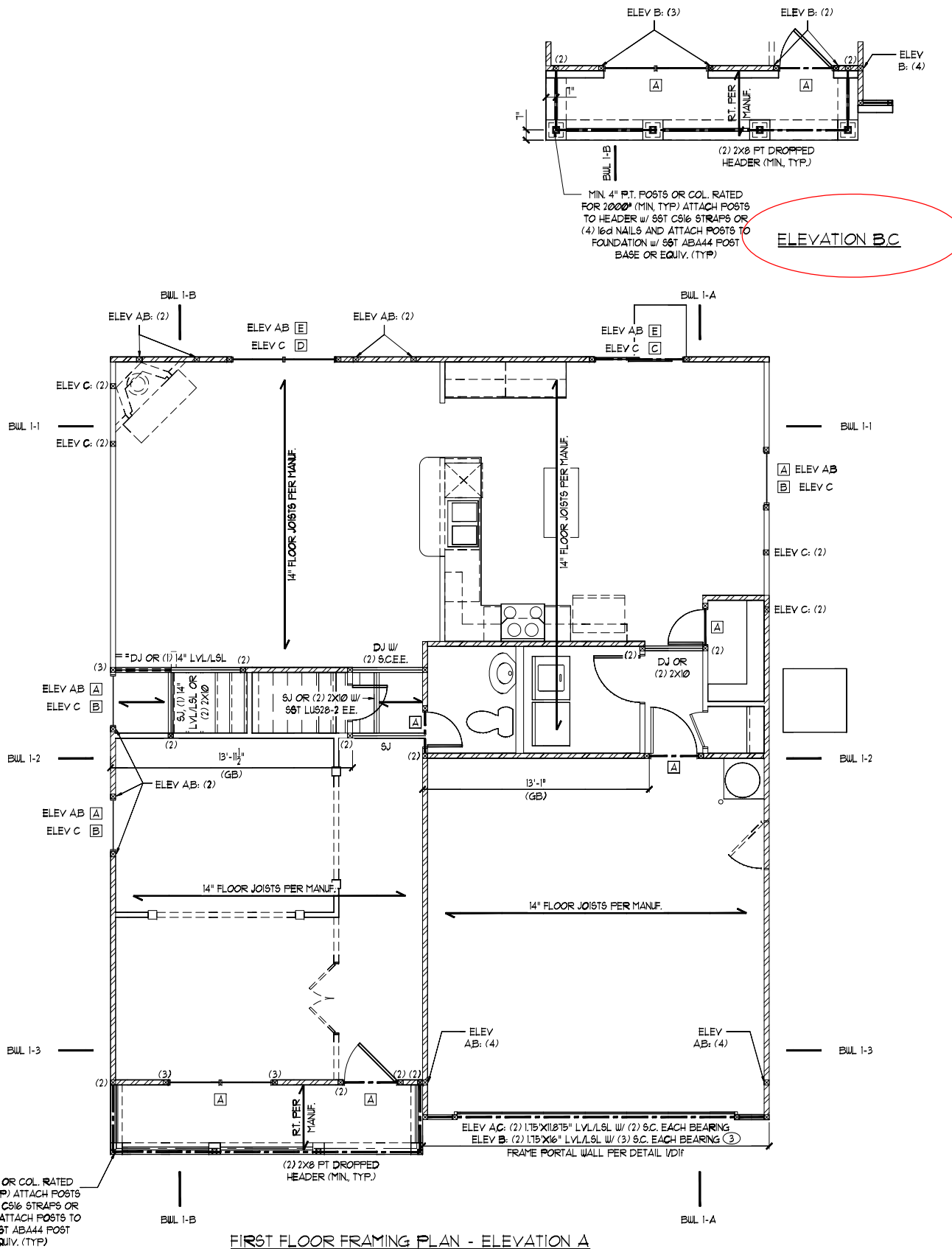
FIRST FLOOR FRAMING PLAN - ELEVATION A
