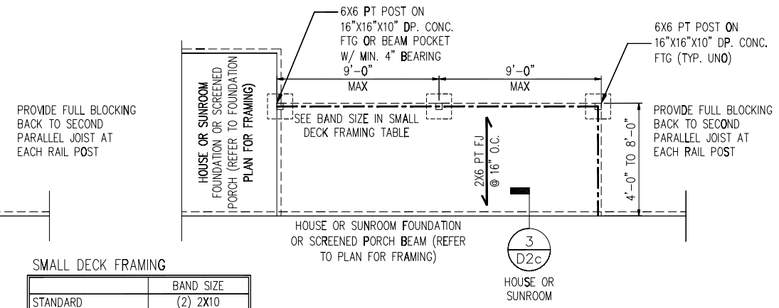
TYP. SMALL SIDE DECK PLAN N.T.S.
