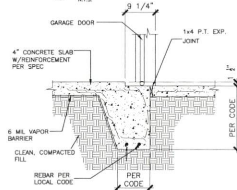
6 TYPICAL GARAGE DOOR DETAIL N.T.S.
