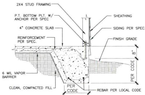
4 TYPICAL SLAB DETAIL N.T.S.
