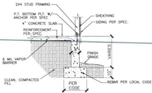
8 TYPICAL STEM WALL DETAIL N.T.S.
