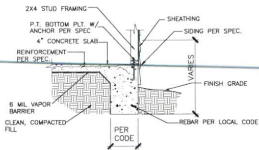
7 TYPICAL TURNDOWN SLAB DETAIL N.T.S.
