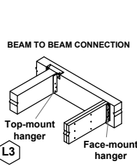
L3 Face-mount hanger
