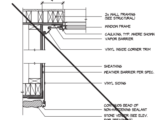
RECESSED WINDOW JAMB - STONE SCALE 1/2"=1'-0" SE-02098g
