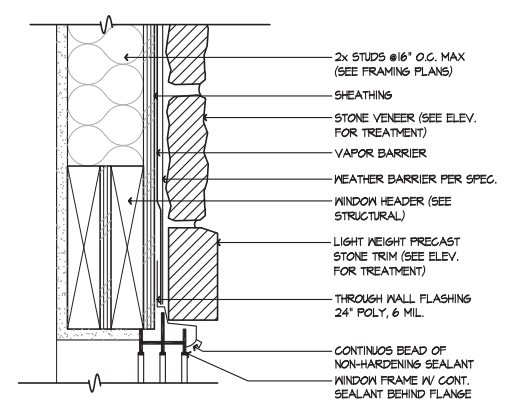
WINDOW HEAD - STONE SCALE 3/8"=1'-0" SE-02096g
