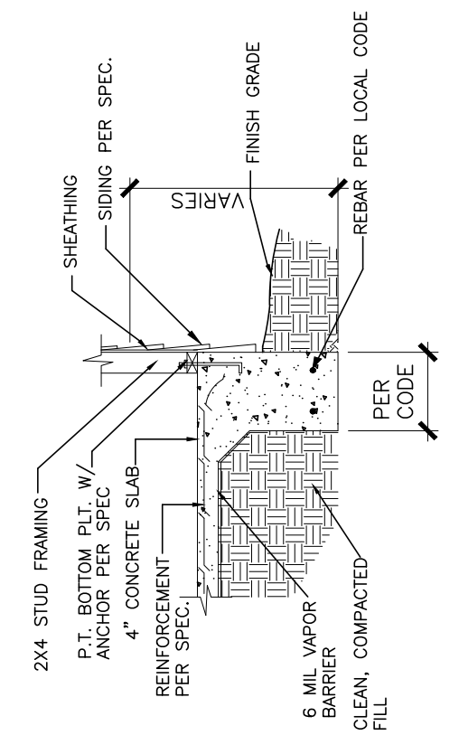
4 TYPICAL SLAB DETAIL N.T.S.
