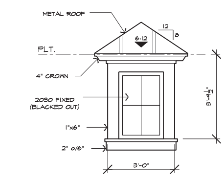
TYP. HIP DORMER NOT TO SCALE
