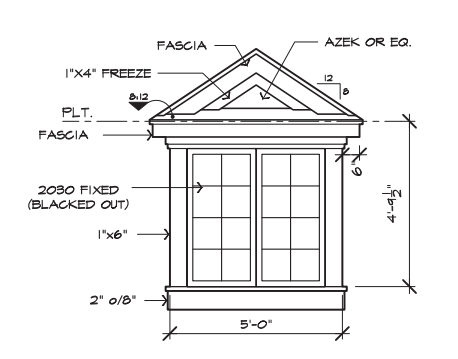
EYEBROW DORMER NOT TO SCALE
