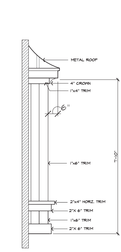
BAY (2) NOT TO SCALE
