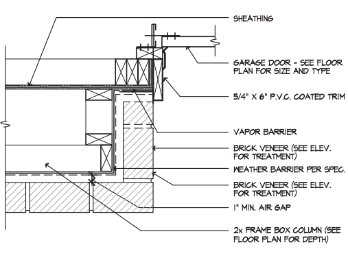
GARAGE DOOR HEAD - BRICK SCALE 1/2"=1'-0" SE-05044a
