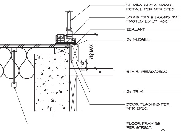
SLIDING GLASS DOOR 157 SCALE 1"=1'-0" AT CRAWL SPACE ADB
