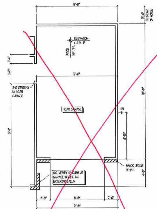
OPT. 1 CAR GARAGE (FWD) SCALE: 1/4" = 1'-0"
