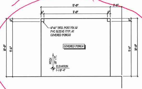
OPT. COVERED PORCH SCALE: 1/4" = 1'-0"
