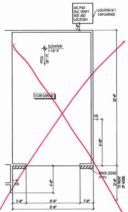
OPT. 1 CAR GARAGE (REAR) SCALE: 1/4" = 1'-0"
