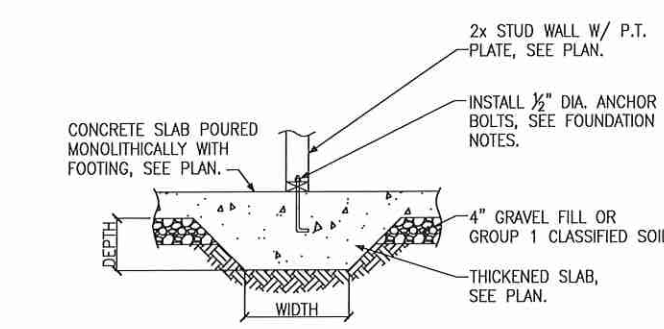
J FOUNDATION SECTION THICKENED SLAB
