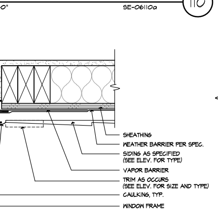
111 WINDOW JAMB - SIDING SCALE 3"=1'-0" SE-06111a
