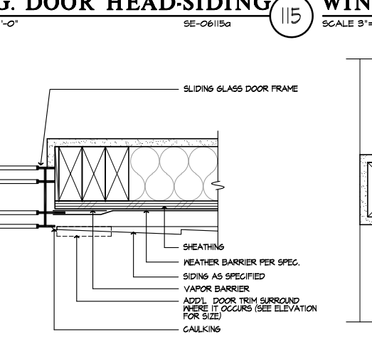
116 SLDG. DOOR JAMB-SIDING SCALE 3"=1'-0" SE-06116a
