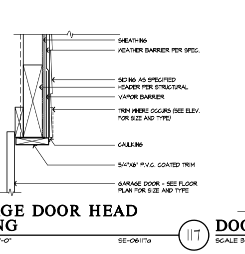
117 GARAGE DOOR HEAD -SIDING SCALE 1/2"=1'-0" SE-06117a
