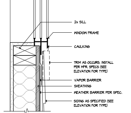
110 WINDOW SILL - SIDING SCALE 3"=1'-0" SE-06110a
