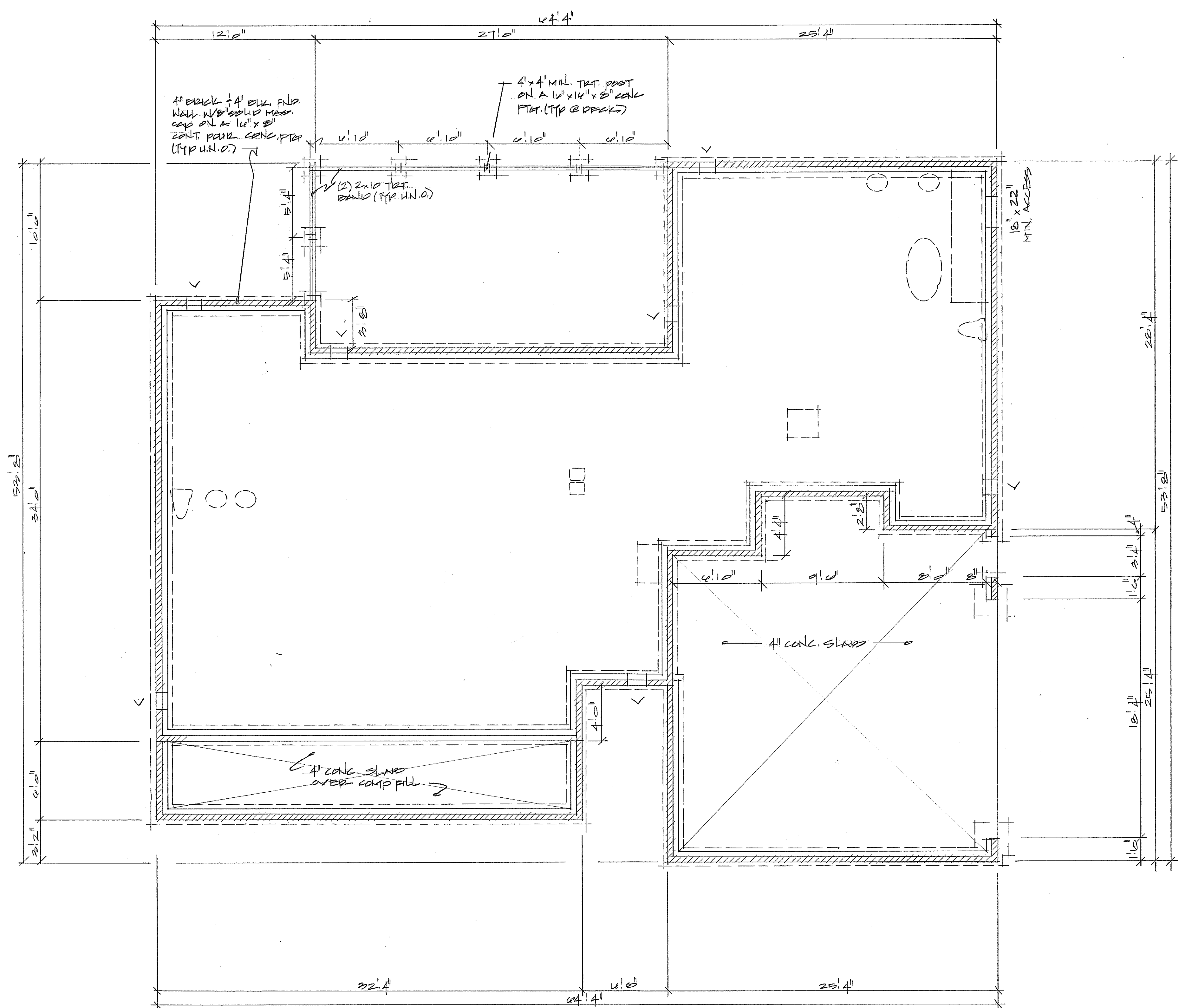
FOUNDATION PLAN @ 1/4" = 1'-0"
