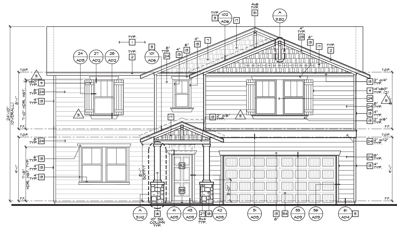
FRONT ELEVATION 'B' AT OPTIONAL 9'-11" PLT. HGT. SCALE 1/4"=1'-0" (22'X34") - 1/8"=1'-0" (11'X17")
