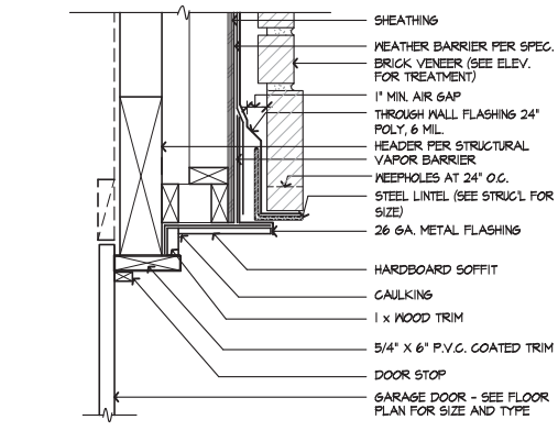
GARAGE DOOR HEAD - BRICK SCALE 1/2"=1'-0" SE-05049a
