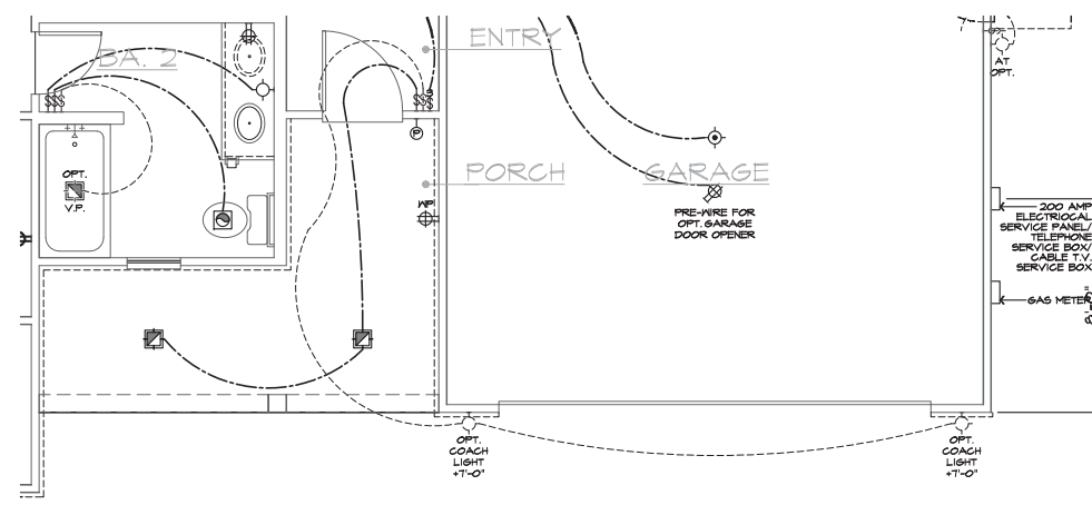
PARTIAL UTILITY PLAN 'B' SCALE 1/4"=1'-0" (22"x34") - 1/8"=1'-0" (11"x17") BASIC PLAN
