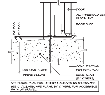
THRESHOLD SCALE 1"=1'-0"
