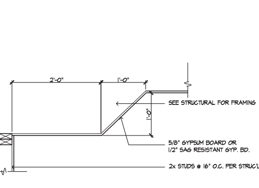
TRAY CEILING SCALE 1"=1'-0" SE-05092a
