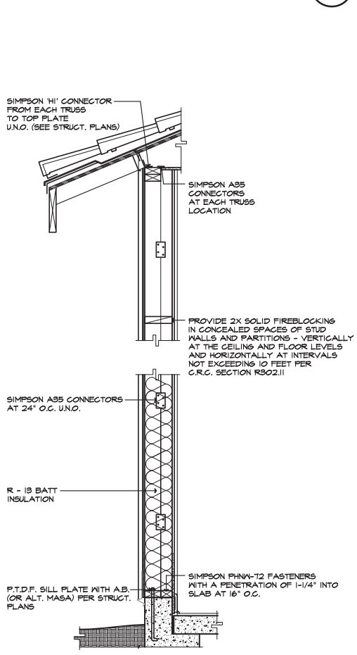
TYPICAL EXTERIOR WALL SCALE 1"=1'-0"
