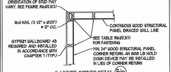
(b) INSIDE CORNER DETAIL ⑤b
