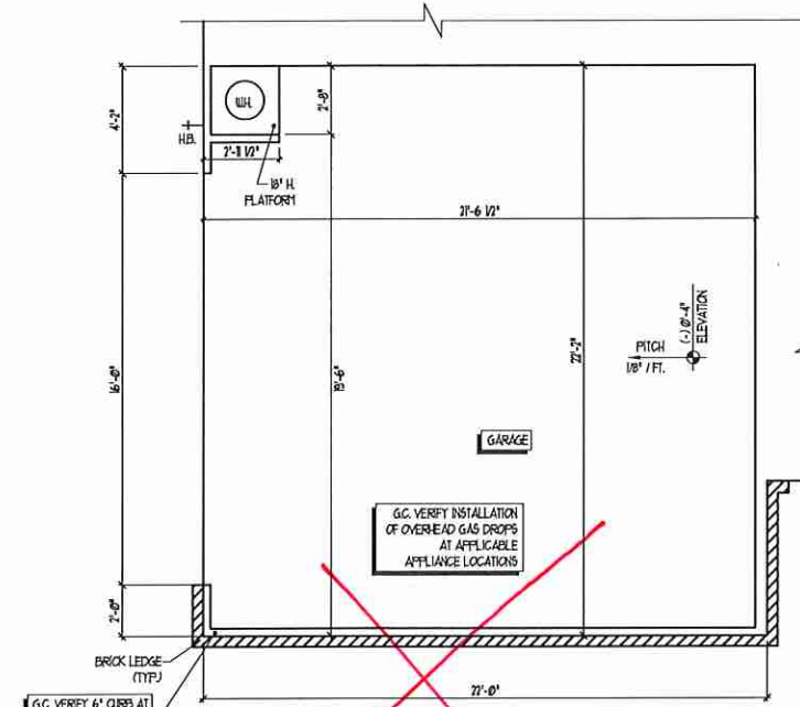
OPT. SIDE LOAD GARAGE SCALE: 1/4" = 1'-0"
