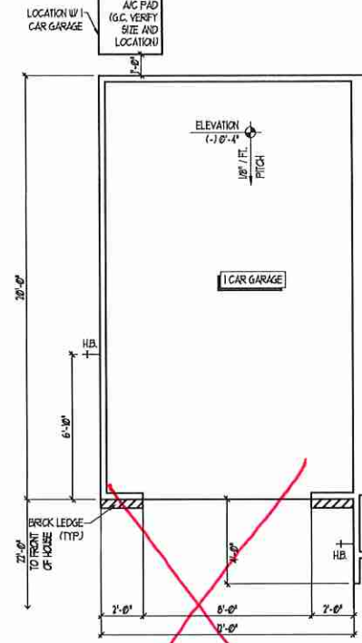
OPT. 1 CAR GARAGE (REAR) SCALE: 1/4" = 1'-0"
