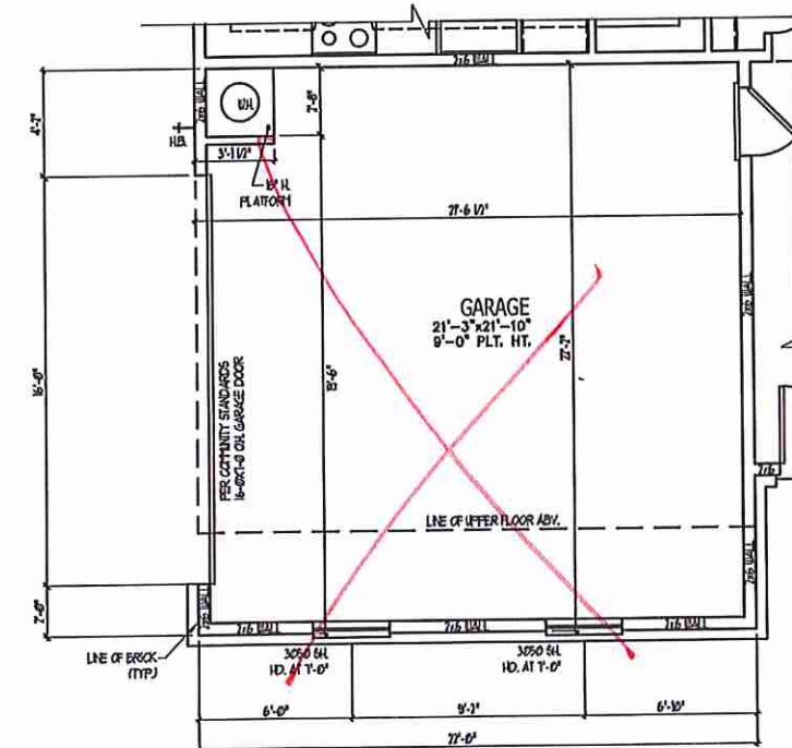
OPT. SIDE LOAD GARAGE
