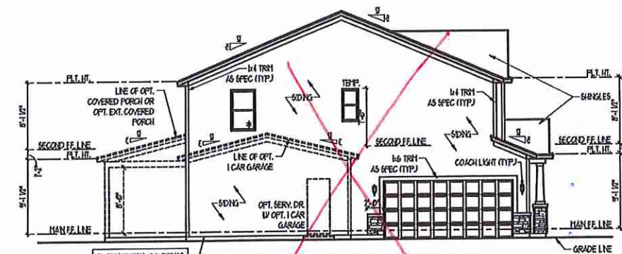
LEFT ELEVATION AT OPT. SIDE LOAD GARAGE SCALE 1/8" = 1'-0"
