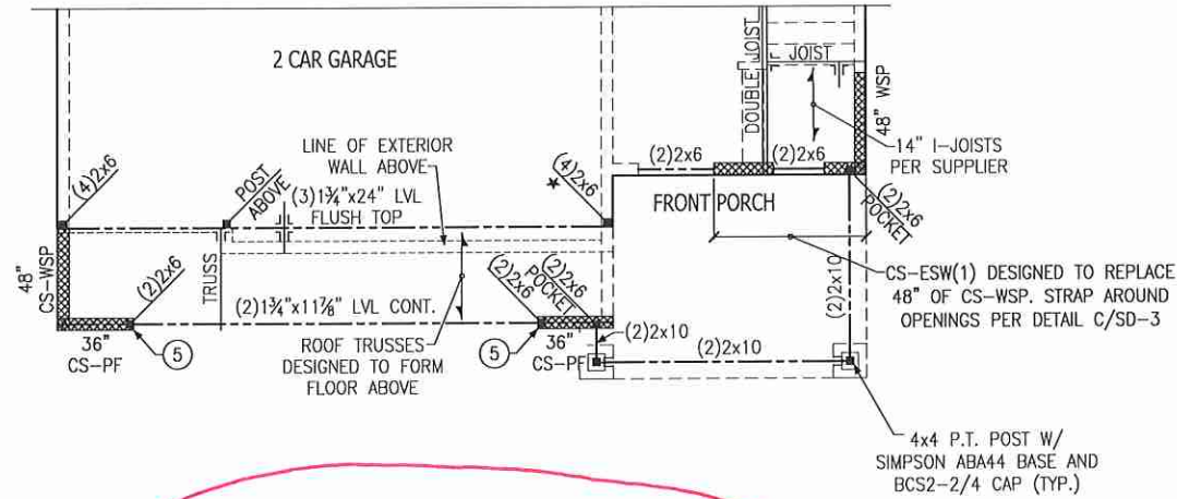
SECOND FLOOR FRAMING PLAN ELEVATIONS 'B1' & 'B2'
