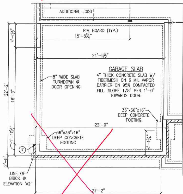
PARTIAL FOUNDATION PLAN OPT. SIDE LOAD GARAGE ELEVATIONS 'A1', 'A2', 'B1' & 'B2'
