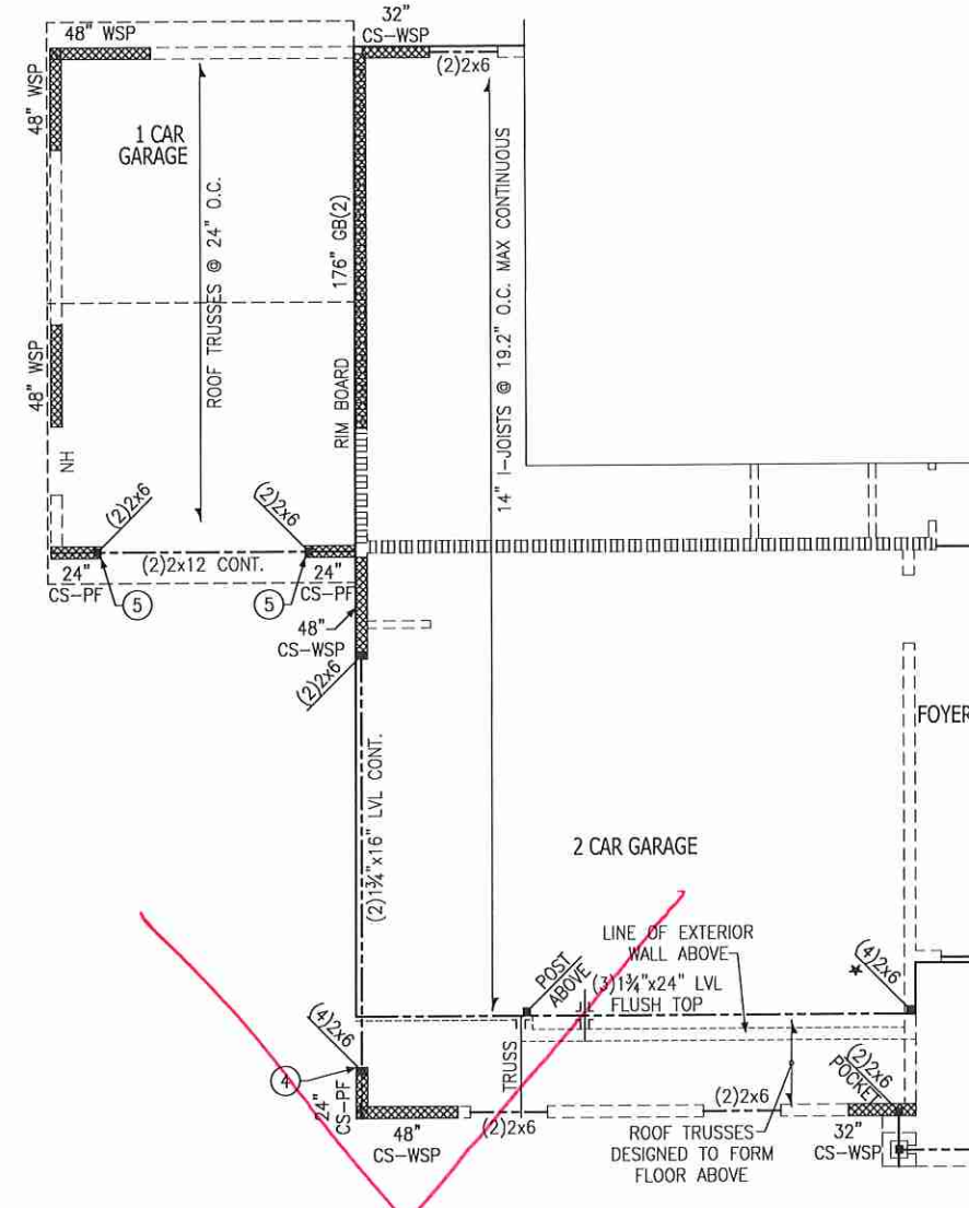
PARTIAL FRAMING PLAN OPT. 3-CAR SWING IN CARRIAGE GARAGE ELEVATIONS 'B1' & 'B2'
