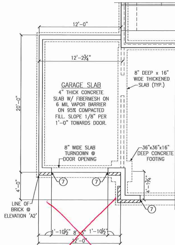
PARTIAL FOUNDATION PLAN OPT. 1 CAR GARAGE ELEVATIONS 'A1', 'A2', 'B1' & 'B2'
