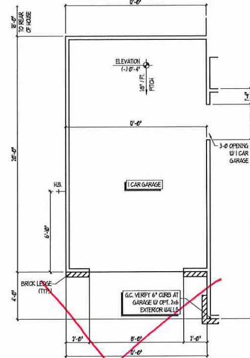
OPT. 1 CAR GARAGE (FWD) SCALE: 1/4" = 1'-0"
