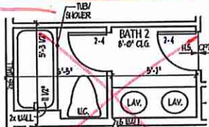
OPT. WALL IN BATH 2 SCALE: 1/4" = 1'-0"
