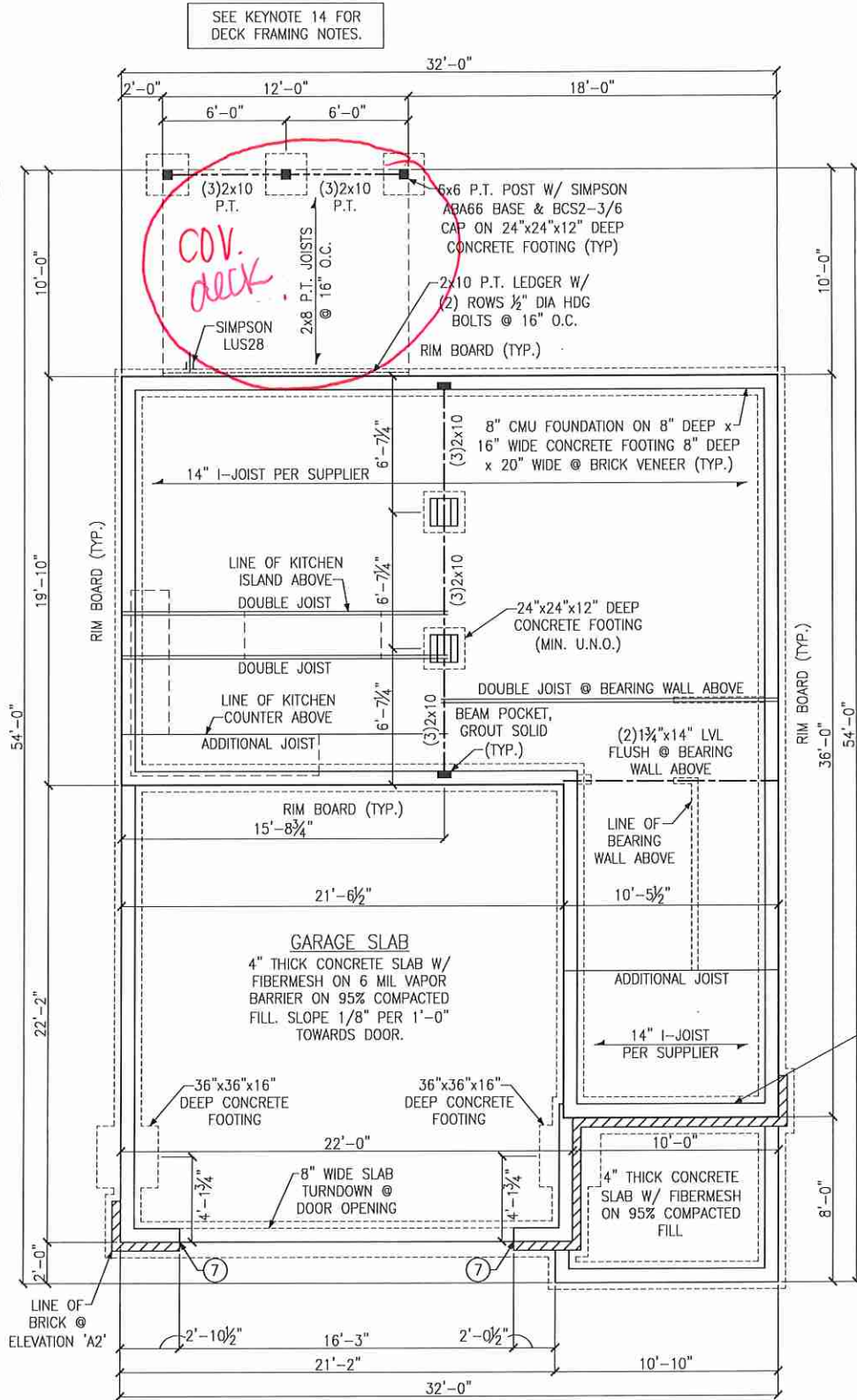
CRAWL SPACE FOUNDATION PLAN ELEVATIONS 'A1' & 'A2'
