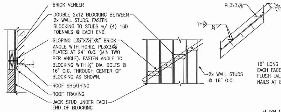
SECTION VIEW
