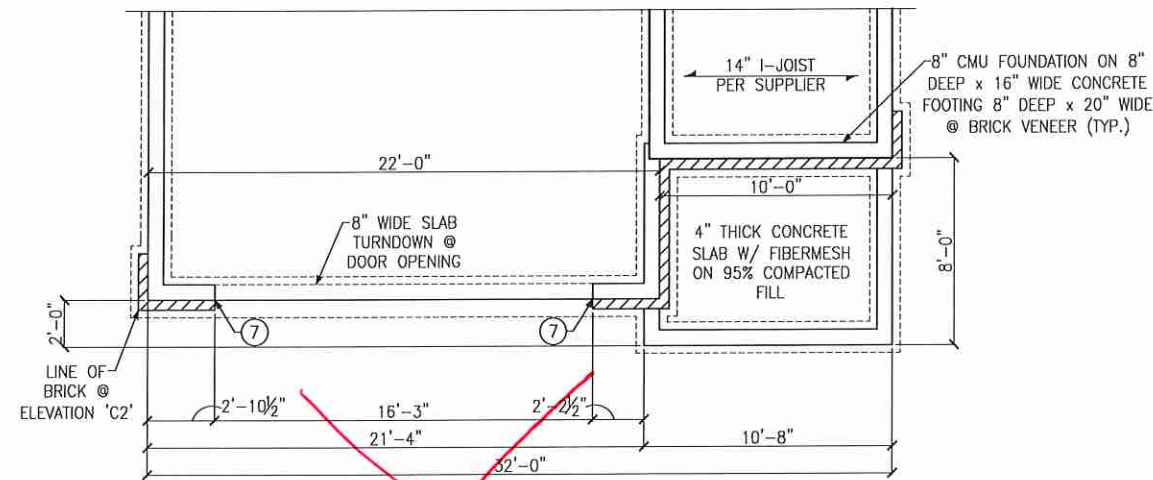
CRAWL SPACE FOUNDATION PLAN ELEVATIONS 'C1' & 'C2'
