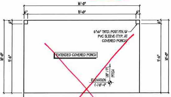
OPT. COVERED PORCH SCALE: 1/4" = 1'-0"
