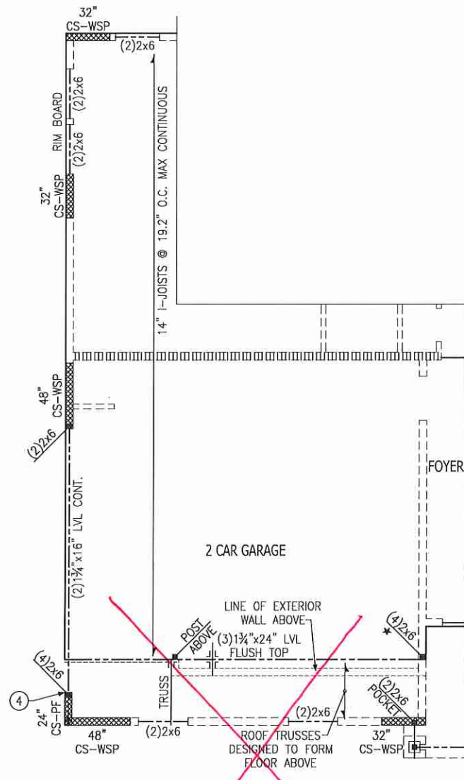
PARTIAL FRAMING PLAN OPT. SIDE LOAD GARAGE ELEVATIONS 'B1' & 'B2'
