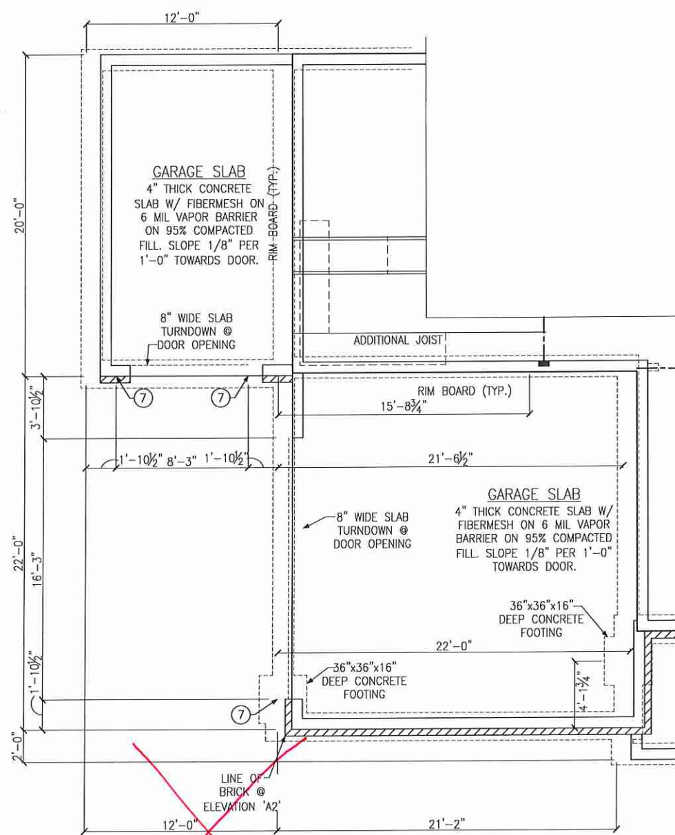
PARTIAL FOUNDATION PLAN OPT. 3-CAR SWING IN CARRIAGE GARAGE ELEVATIONS 'A1', 'A2', 'B1' & 'B2'
