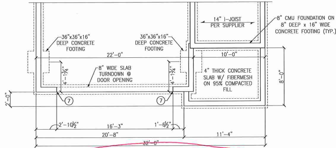
CRAWL SPACE FOUNDATION PLAN ELEVATIONS 'B1' & 'B2'
