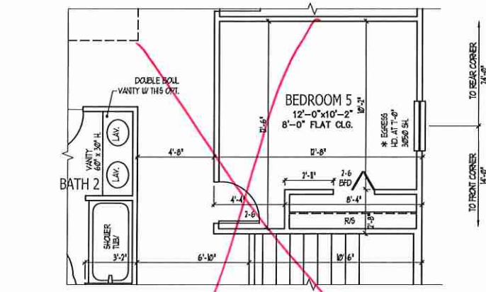
OPT. BEDROOM 5 I.L.O. LOFT SCALE: 1/4" = 1'-0"
