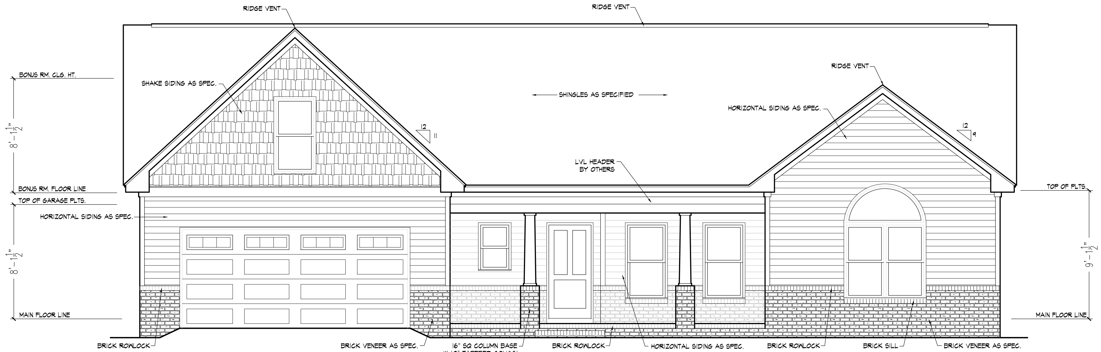
101 Front Elevation
