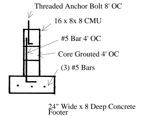
Detail 1 Footer and Perimeter Foundation Wall
