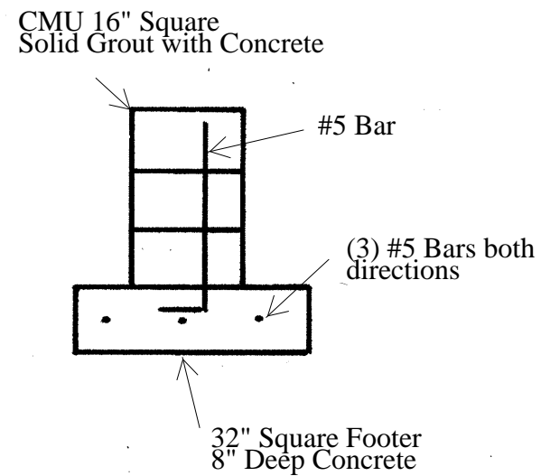
Detail 2 Pier
