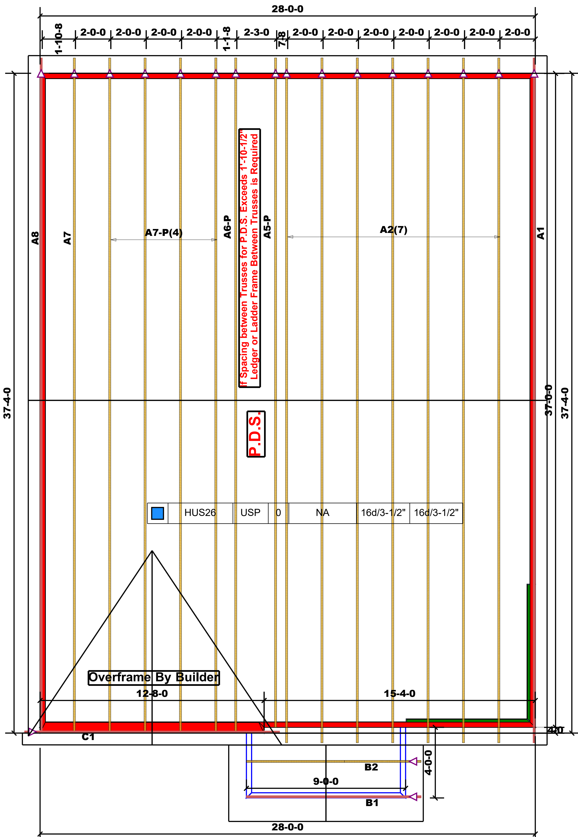
Truss Placement Plan SCALE: NTS
