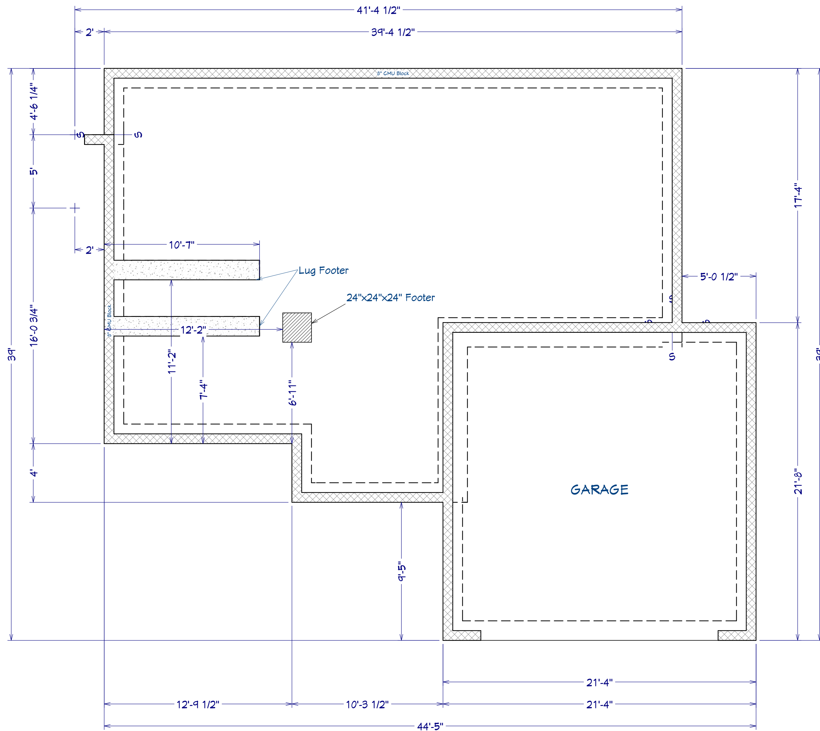
Foundation FOUNDATION PLAN Scale: 1/4" = 1'0"
