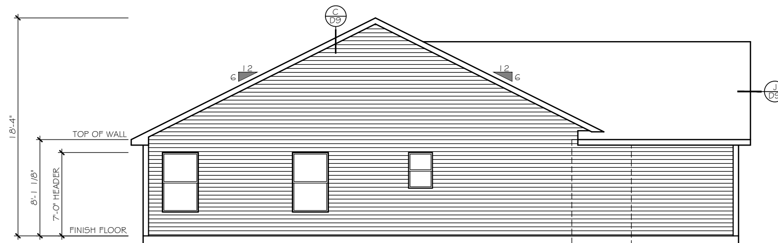
LEFT ELEVATION
