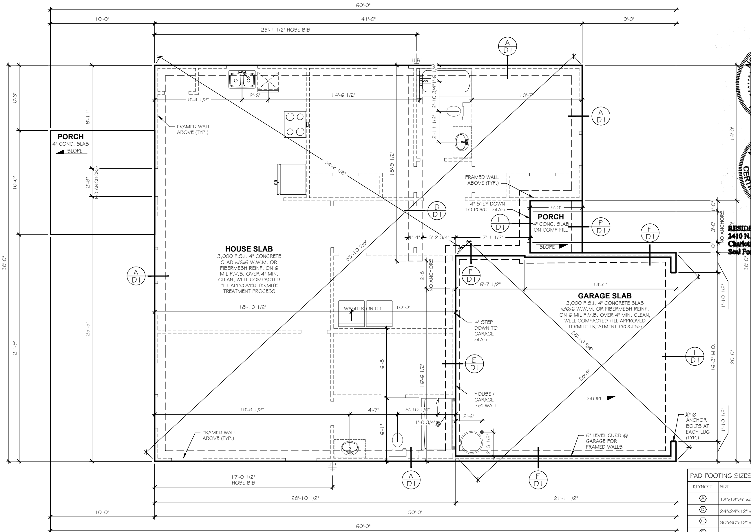
MONO SLAB FOUNDATION PLAN
