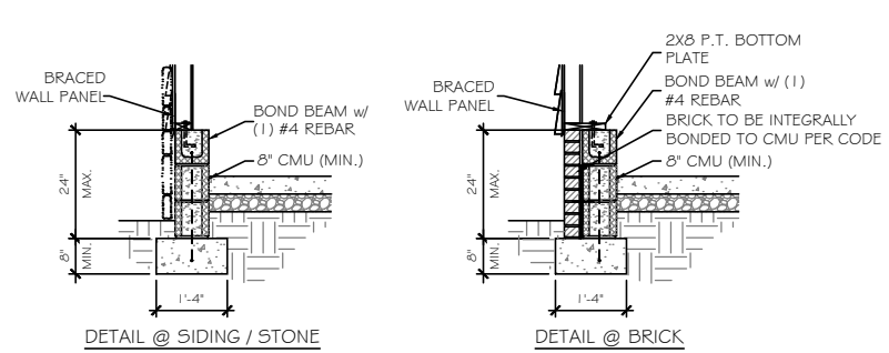
C MASONRY STEM WALL SUPPORTING BRACED WALL PANEL DETAILS
