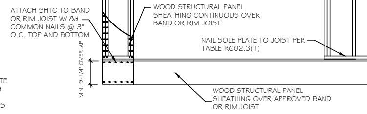
B OVER RAISED WOOD FLOOR - OVERLAP OPTION
