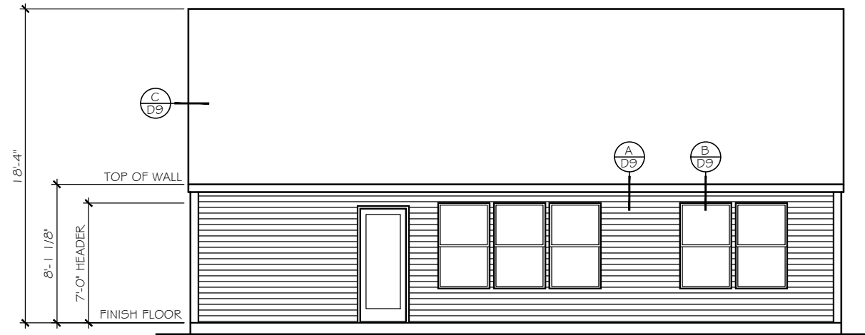
REAR ELEVATION
