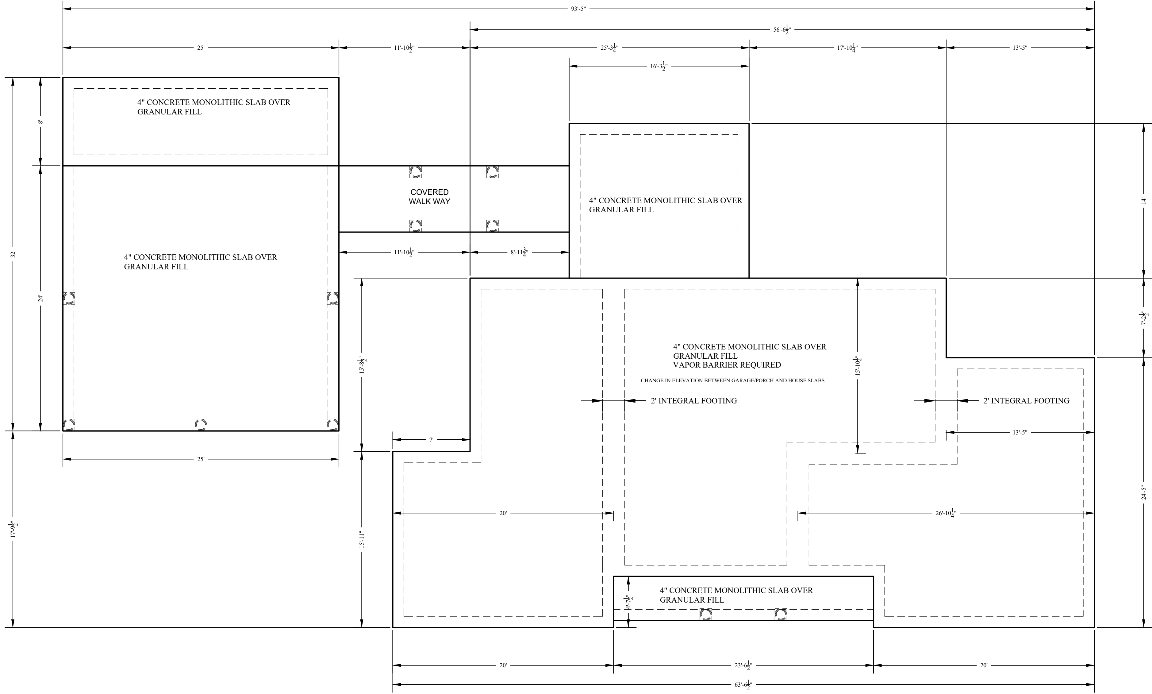
FOUNDATION PLAN 3/16"=1'-0"
