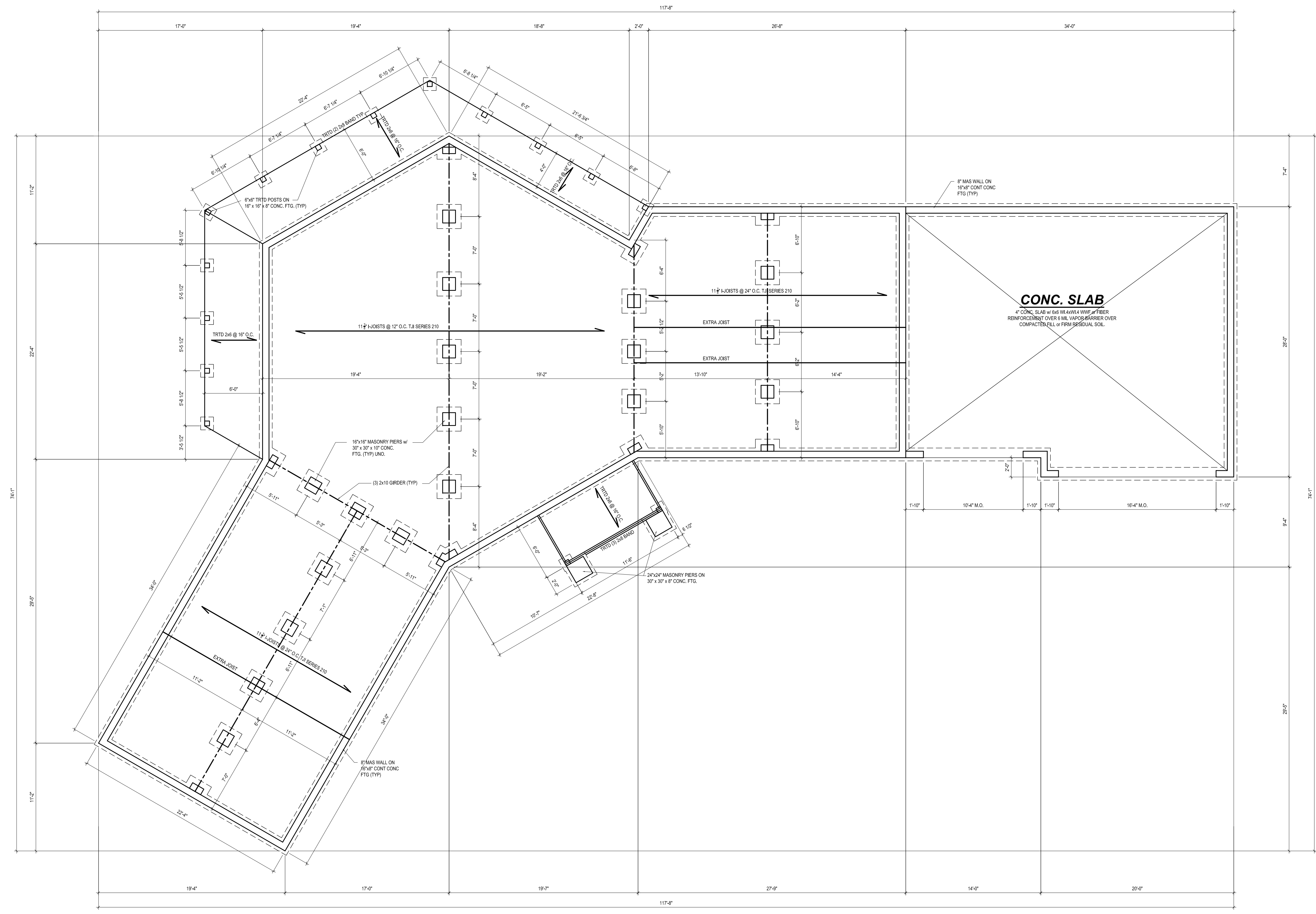
FOUNDATION PLAN
