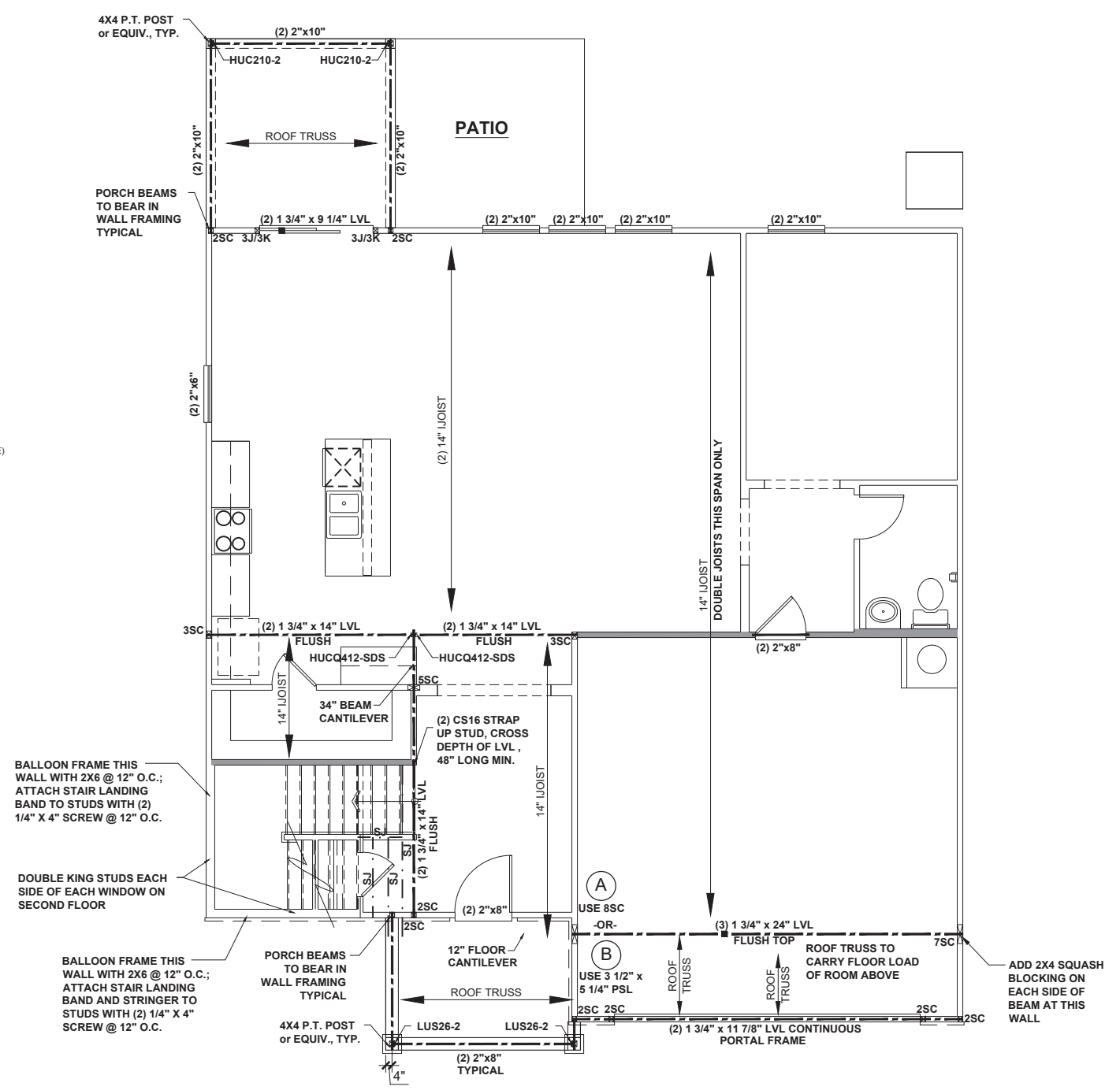
FIRST FLOOR CEILING FRAMING PLAN - 'C' SCALE: 1/8"=1'-0"
