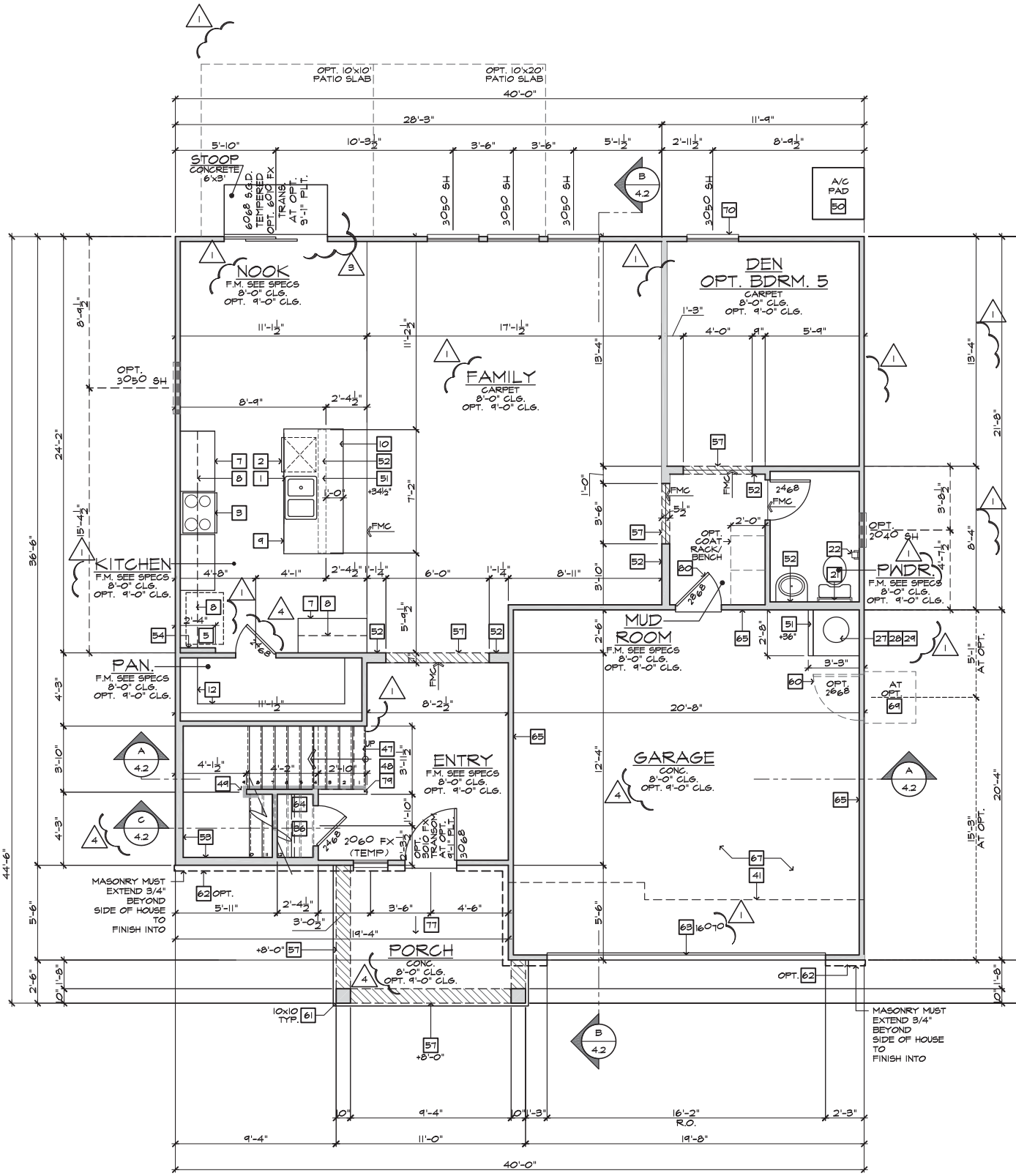
FIRST FLOOR PLAN 'A' SCALE 1/4"=1'-0" (22"X34") - 1/8"=1'-0" (11"X17") BASIC PLAN
