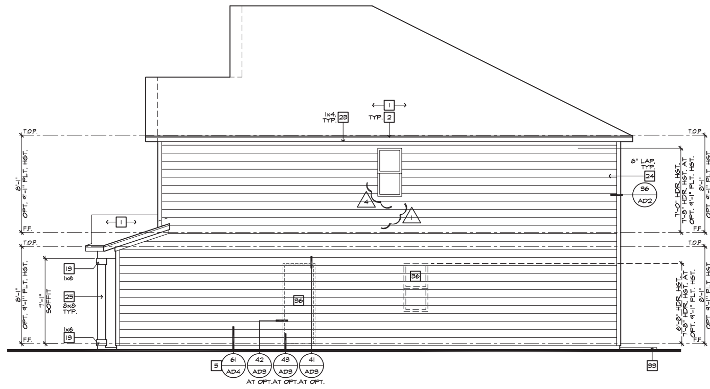
RIGHT ELEVATION 'C' SCALE 1/4"=1'-0" (22'x34') - 1/8"=1'-0" (11'x17')
