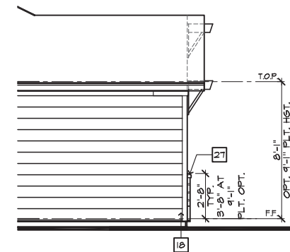
PARTIAL LEFT ELEVATION 'B' W/ MASONRY OPTION
