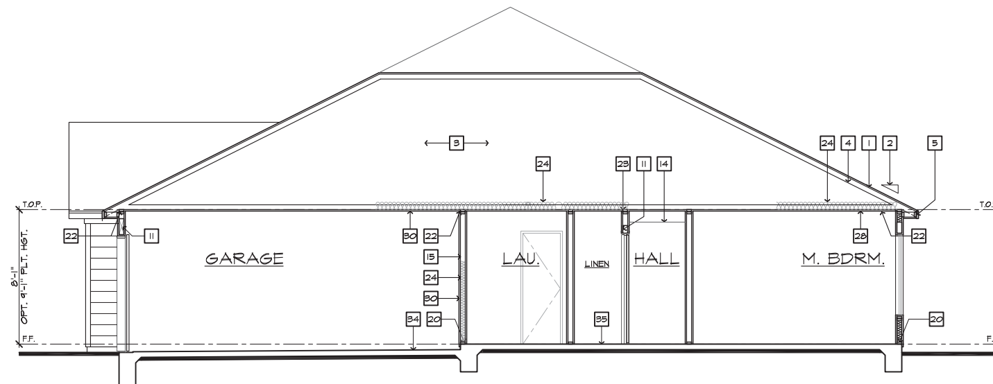
SECTION "B"
