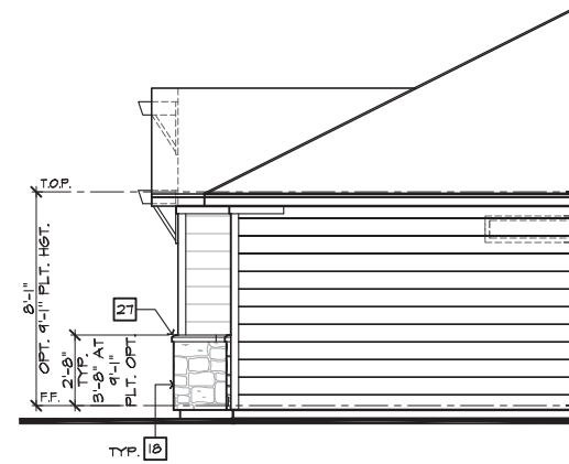
PARTIAL RIGHT ELEVATION 'B' W/ MASONRY OPTION
