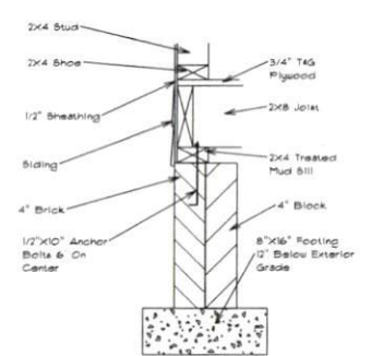
Foundation Detail
