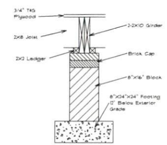
Footing & Pier Detail
