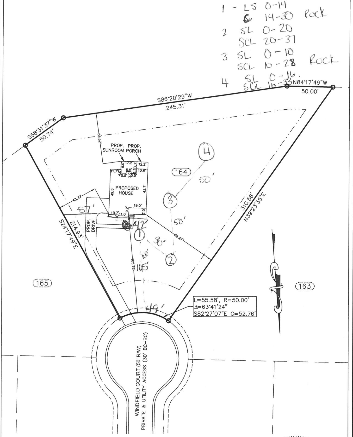
PLOT PLAN
