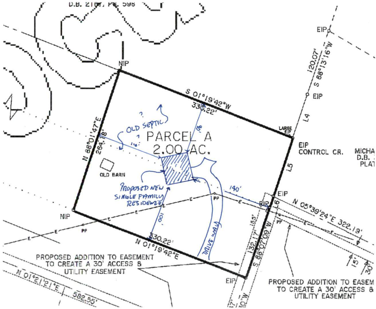
SITE PLAN 1" = 100'-0"
